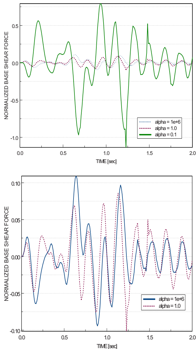
Fig. 5. (a) Base shear-force response of a rigid dam facing a headwater height of h=65 m, when subjected to the selected portion of the Taft earthquake accelerogram, N21E component (July 1952), for several values of the reservoir bottom impedance ratio \alpha ; (b) contrasting two of the base shear-force responses in (a): for a very stiff reservoir bottom ( \alpha=1e+6 ) versus the same response for an almost-water reservoir bottom ( \alpha=1.0 )
