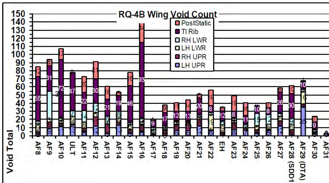
Figure 5. Wing Void Count by Airframe
