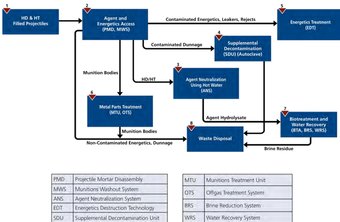
Figure 3. Schematic of the Neutralization Process at the PCAPP Facility
