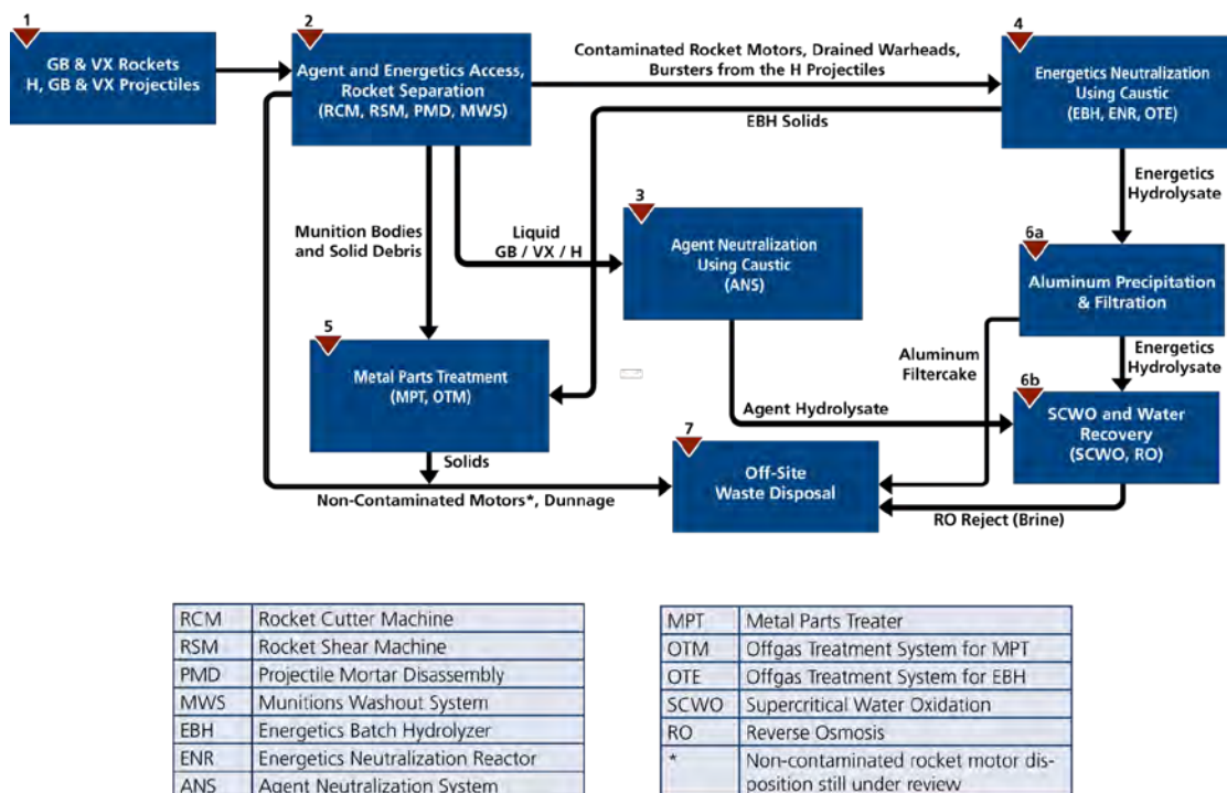
Figure 4. Schematic of the Neutralization Process at the BGCAPP Facility
