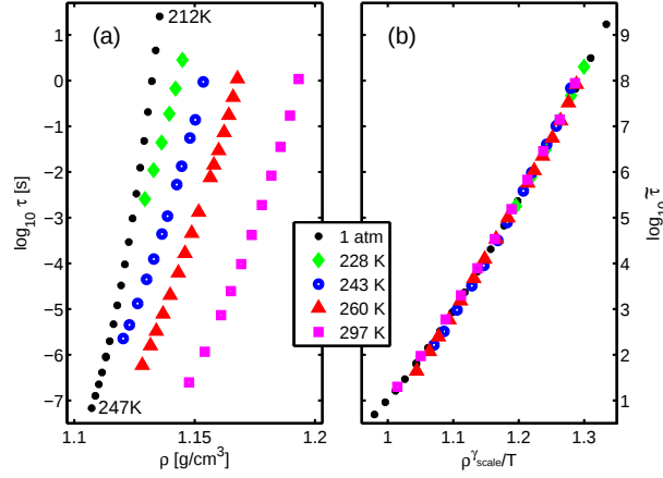
FIG. 1: The dielectric relaxation time \tau measured along different isotherms and along the atmospheric pressure isobar for the silicone oil DC704. The points come from measured loss peaks and the relaxation times refer to inverse angular loss-peak frequencies. (a) The relaxation times as functions of density (calculated from measured pVT-data). (b) The reduced unit relaxation time, \tilde{\tau} = C\rho^{1/3}T^{1/2}\tau , as a function of K\rho^{\gamma_{\text{scale}}}/T , where \gamma_{\text{scale}} = 6.2 \pm 0.2 is a parameter adjusted to collapse the data of (a). C and K are constants which have no influence on the quality of the scaling, they only shift the axes.
