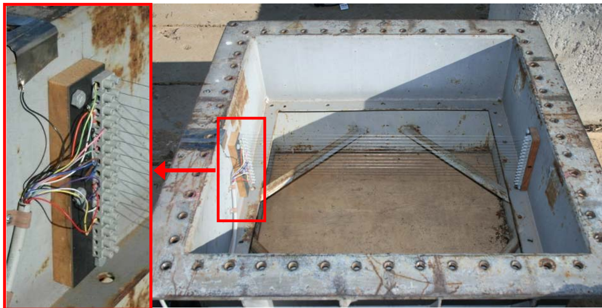
Figure 8 Wire displacement measurement system as set up before the blast event
