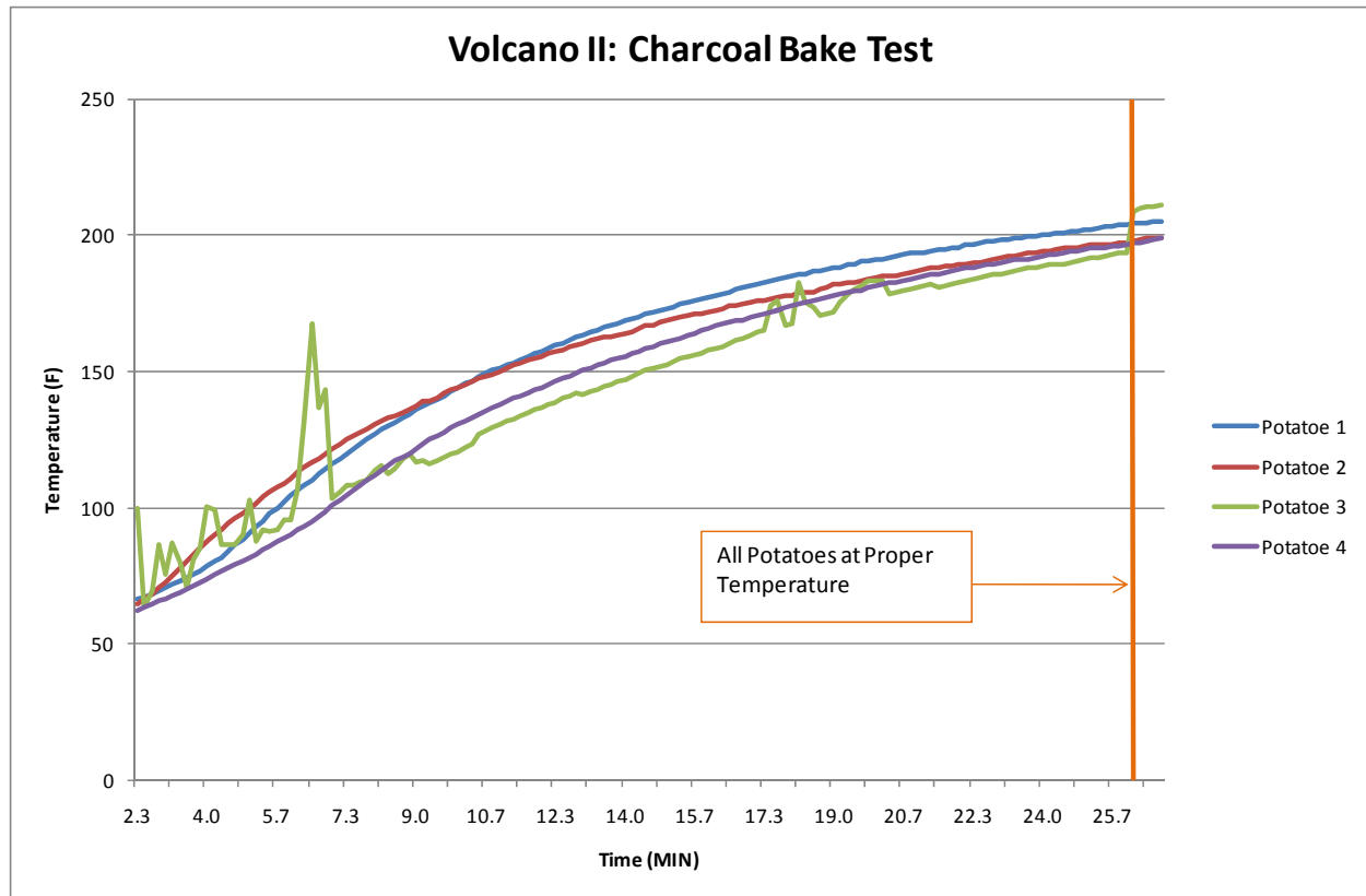
Figure 21. Charcoal Baking Test Results
