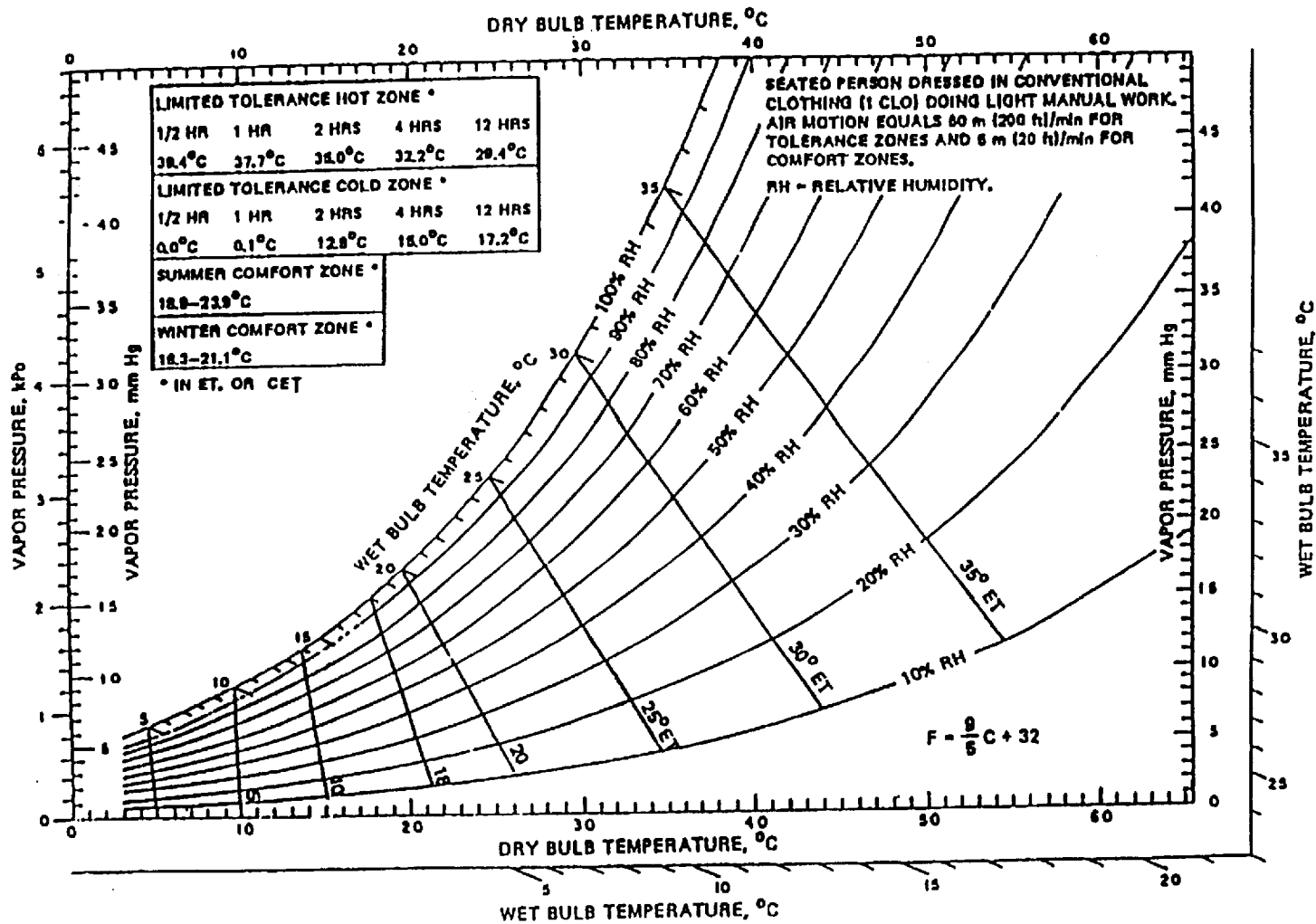
FIGURE. 36 Summer and winter comfort zones and thermal tolerance for inhabited compartments
