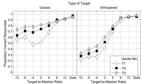
Figure 2: Proportion correct target identification as a function of TMR for voiced (left panel) or whispered (right panel) corpus. The circles represent performance for listeners in conditions where the masker is the same talkers (TT) as the target, the squares represents performance in a condition when the masker is the same-sex talker (TS) as the target, and diamonds show performance in conditions when the target and masker are two different sex talkers (TD). The error bars represent the 95% confidence intervals around the mean.
