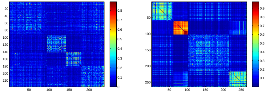
Figure 6.8: Reordered similarity matrices of ‘argument’ (left) and ‘circuit’ (right). These figures show the similarity matrices of the concepts of the words ‘argument’ and ‘circuit’. The components of the matrix are permuted according to the clusterings. The block-diagonal structure of the matrices can clearly be seen.
