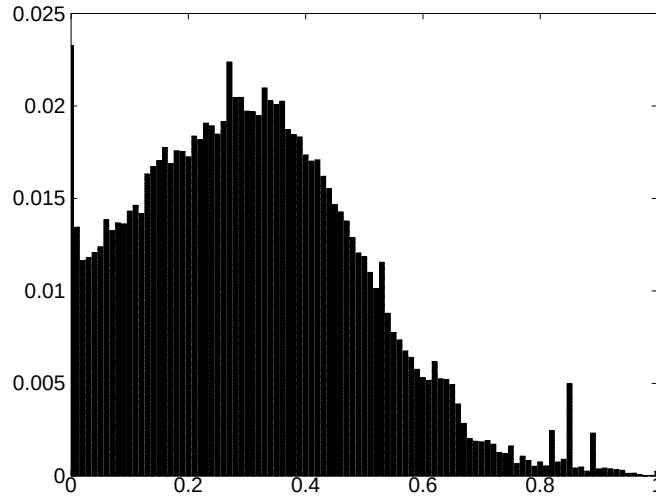
Figure 4.7: A histogram of the distribution of similarity values on links We have taken the graph of 1.5 million webpages where the nodes are the pages, and the edges are the links between them. We have compared all pairs of webpages with a link between them by the cosine distance of their Bag of Words representation. The similarity values are on the horizontal, their relative frequency on the vertical axis. The first bin contains all the values v with 0 \leq v < 0.01 , etc. It can be seen that most of the links have a low similarity value; the distribution is skewed to the right. Based on this data, we can not say that a link from one document to the other implies that they share significant content.
