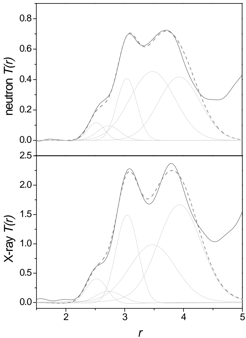
Figure 6: Fits to x-ray and neutron correlation functions for \text{Ca}_{60}\text{Mg}_{20}\text{Cu}_{20} . (The continuous line shows the experimental data, whilst the dashed line shows the fitted function, and the dotted lines show the components of the fit).
