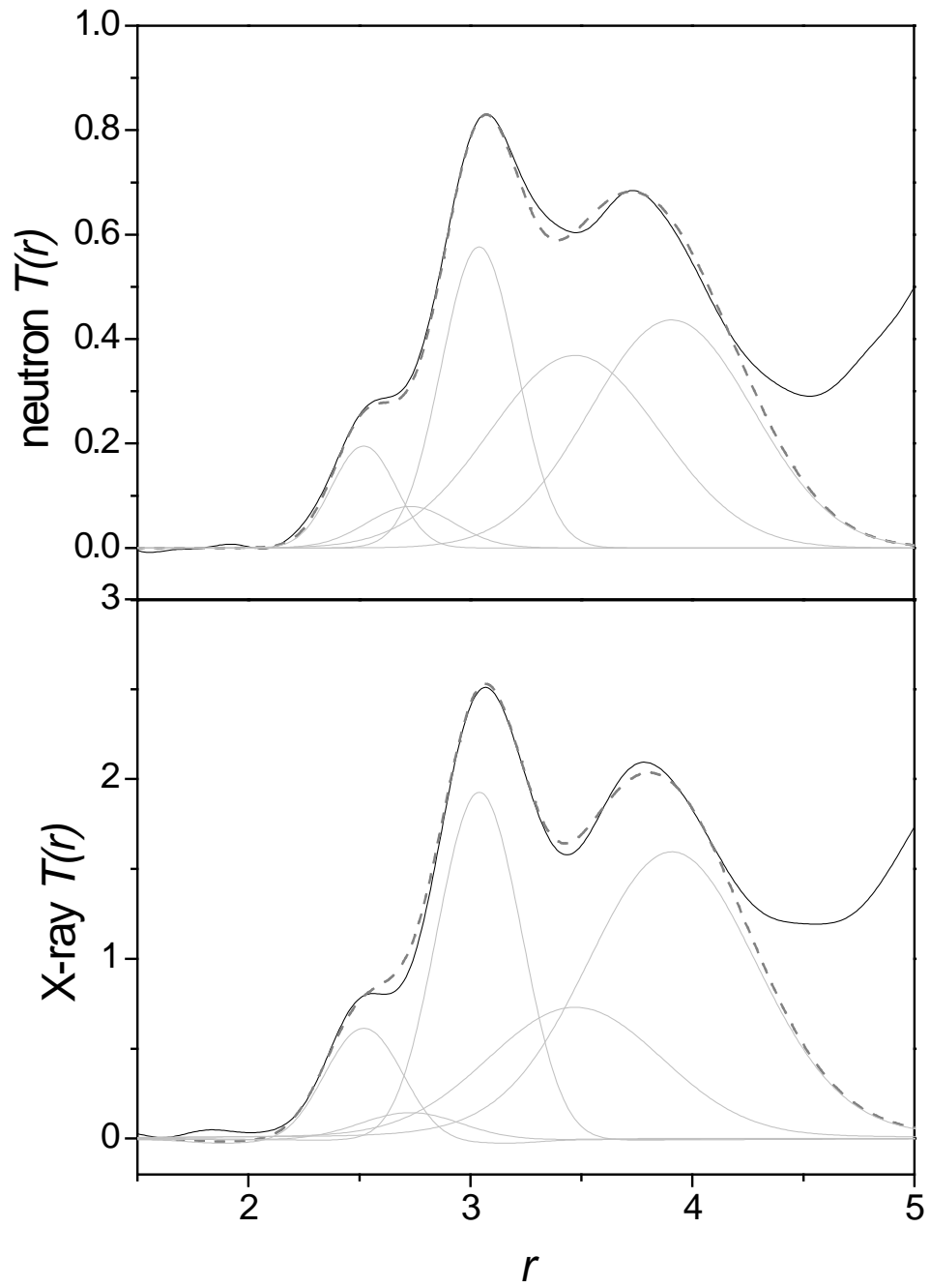
Figure 5: Fits to x-ray and neutron correlation functions for \text{Ca}_{60}\text{Mg}_{15}\text{Cu}_{25} . (The continuous line shows the experimental data, whilst the dashed line shows the fitted function, and the dotted lines show the components of the fit).
