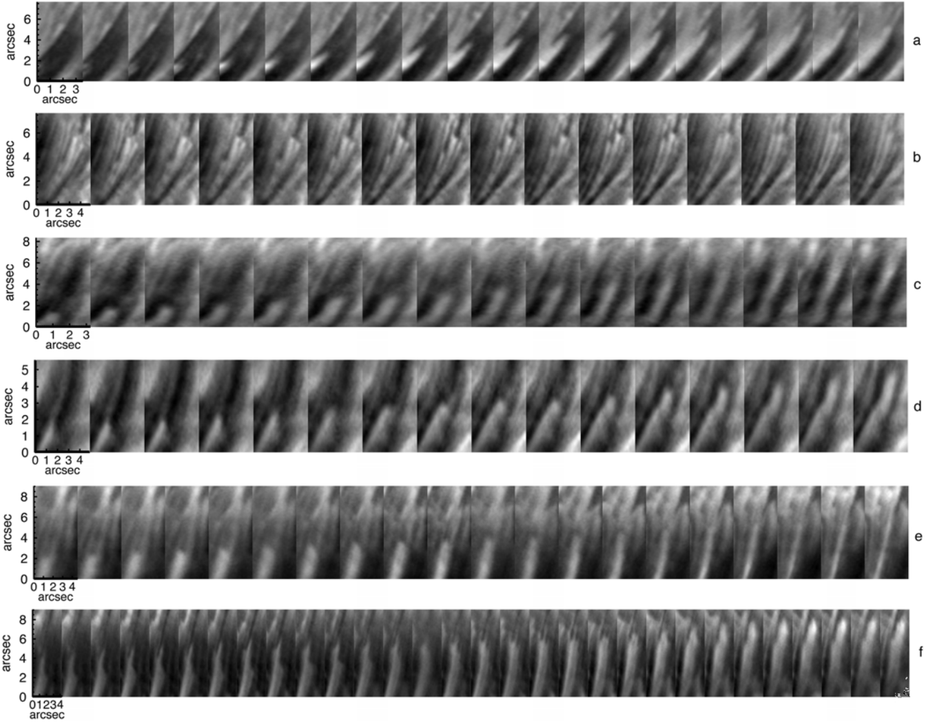
Fig. 2. Six examples of H\alpha jets observed within the white rectangle in the lower left panel of Fig. 1. Each successive image is separated by a time of 8.4 s, while the length of the jet structures range between approximately 3000–6000 km.
