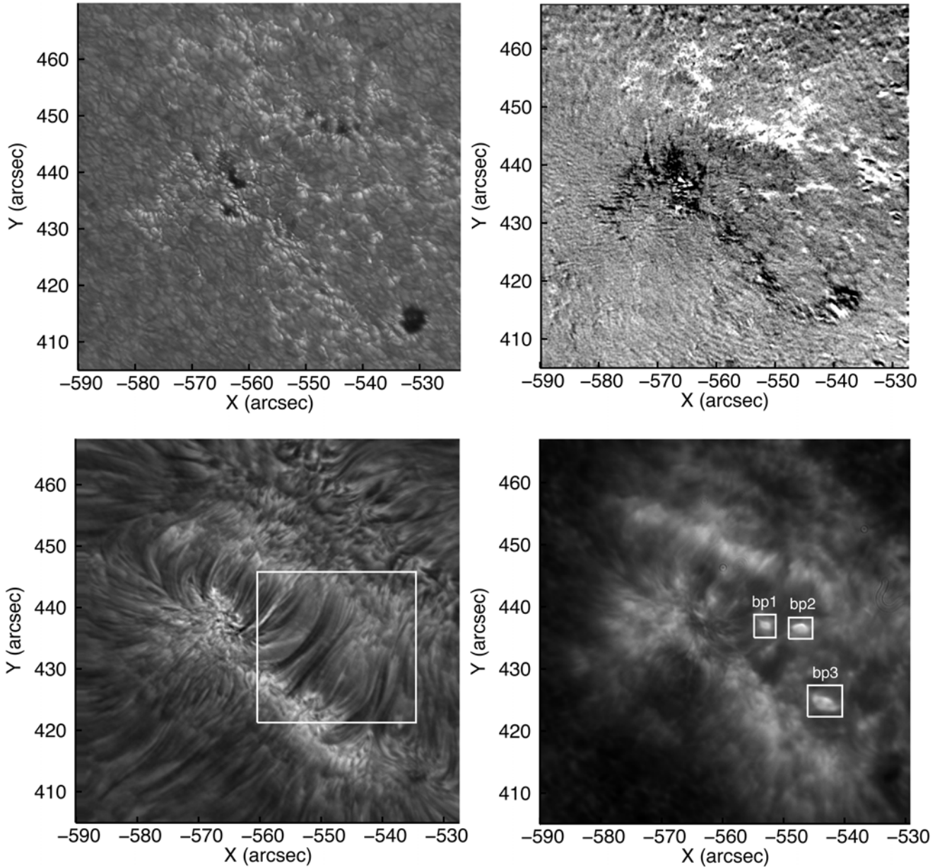
Fig. 1. Simultaneous ROSA images of the G band ( top left ), line-of-sight magnetogram ( top right ), H\alpha core ( bottom left ), and Ca\ II\ K core ( bottom right ). The magnetogram colour scale is in Gauss, where white indicates positive magnetic polarities, while black demonstrates polarities which are negative. Artificial saturation at \pm 400 G is implemented to highlight regions of weak magnetic polarity on the solar surface. The white rectangle in the H\alpha core image indicates the approximate position where most of the jets are observed. White rectangles in the Ca\ II\ K image, identified by “bp1”, “bp2”, and “bp3”, are the bright points selected for temporal analysis. Axes are in heliocentric arcseconds, where 1'' \approx 725 km.
