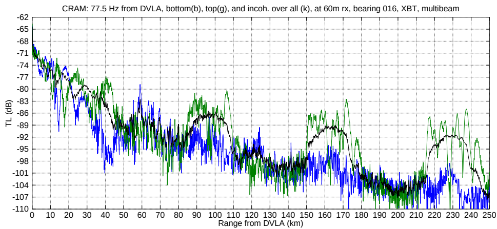
Figure 21 Transmission Loss Versus Range for the 250km Long Line Transmission loss versus range for the 250km long line using PE-CRAM.
