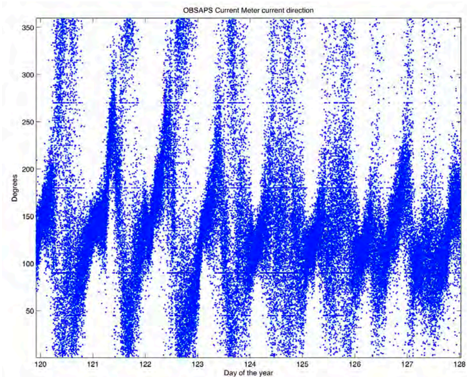
Figure 15 Sample of Seafloor Current Meter Data
