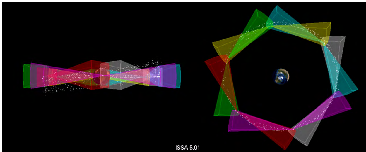
Figure 6 A notional commercially-hosted architecture using six hosts equally spaced 60^\circ along the GEO belt. Each host has two telescopes with a 20^\circ \times 20^\circ FOV, with the optical axis pointing 20^\circ inward relative to the velocity/anti-velocity direction. The positions of GEO space objects from space-track.org are shown.
