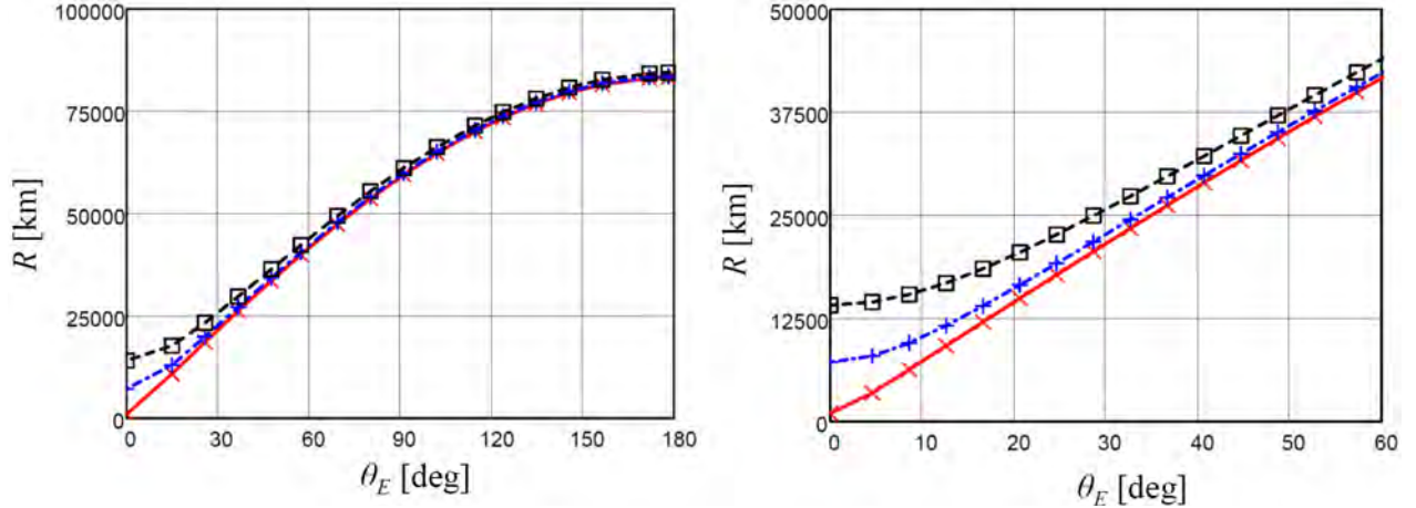
Figure 2 The range to other GEO objects (y-axis, km) as a function of the “belt angle”, \theta_E (x-axis, degrees). The \times , + , and \square lines correspond to a declination angles ( \theta_{DEC} ) of 0^\circ , 10^\circ , and 20^\circ . At left, the full range around the belt is shown, while the figure on the right is restricted to \theta_E < 60^\circ .
