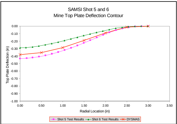
Figure 2. SAMSI Simulation Results Versus Test Results
