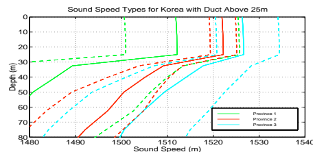
Provinced sound speed profiles without and with a duct
