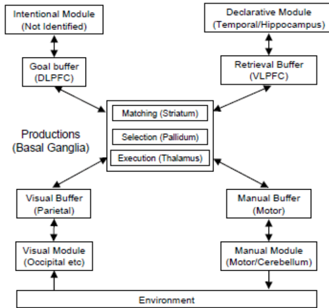
Figure 7: Architecture of ACT-R (Anderson et al., 2004; Chong et al., 2007)
