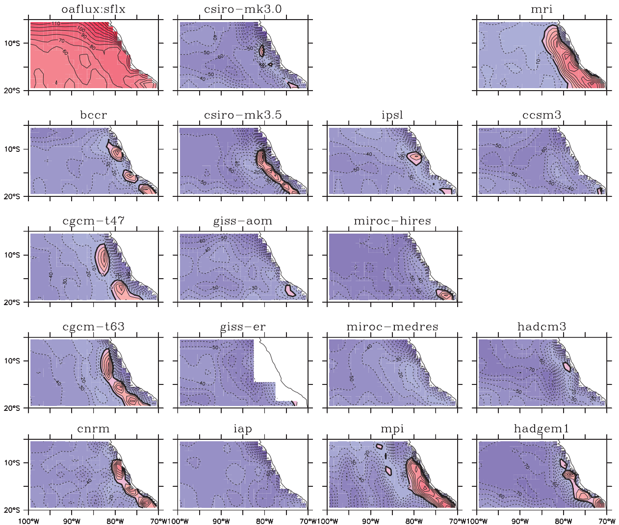
FIG. 3. Spatial distribution of the net surface heat flux biases (shading contours; \text{W m}^{-2} ) relative to OAFlux from 17 IPCC AR4 coupled GCMs in the region ( 20^{\circ} – 5^{\circ}\text{S} , 100^{\circ} – 70^{\circ}\text{W} ) of the SEP: (top left) net surface heat flux from OAFlux.
