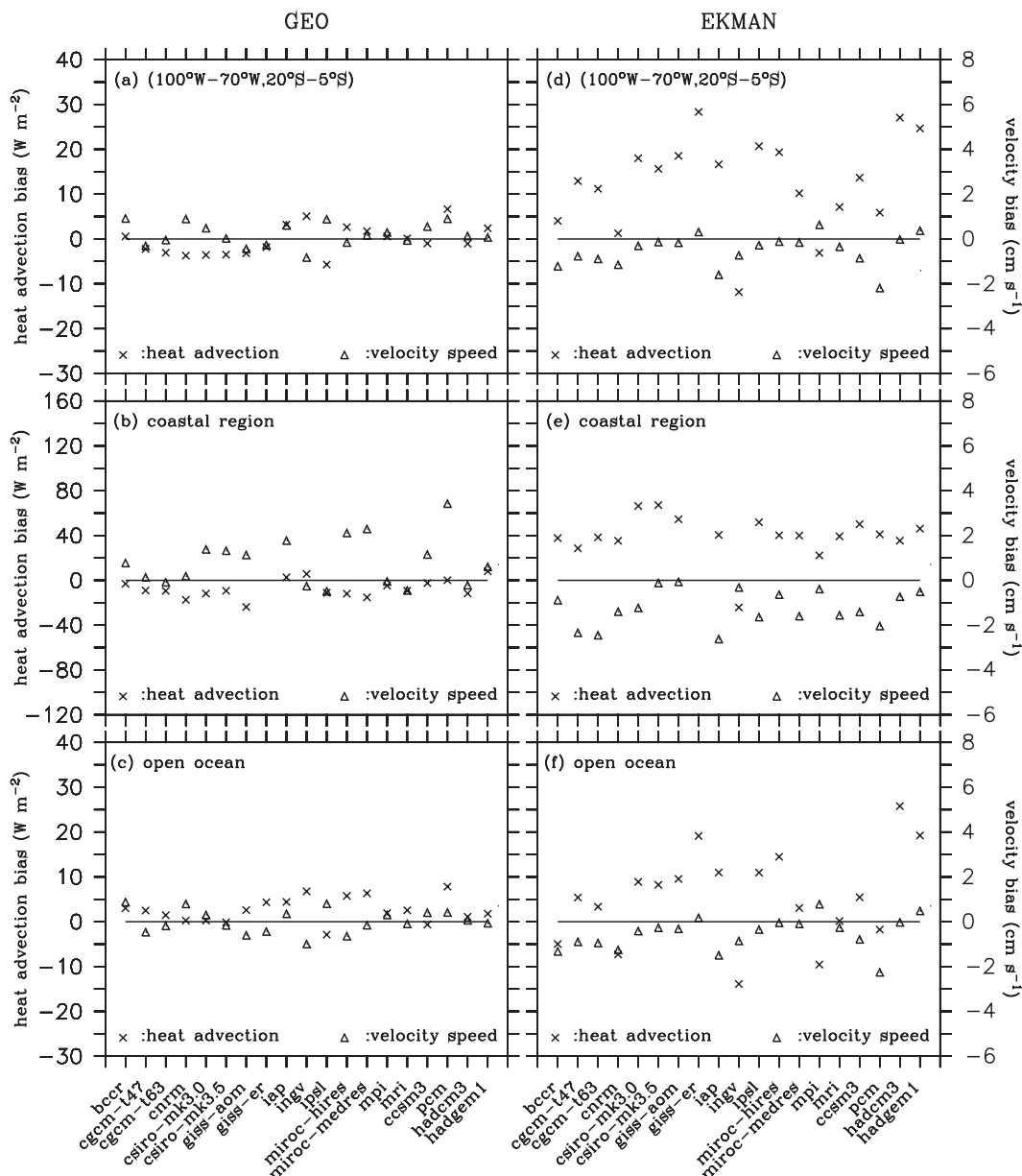
FIG. 11. Biases of geostrophic heat advection (denoted by “x”; \text{W m}^{-2} ) and biases of geostrophic current speed (denoted by “ \Delta ”; \text{cm s}^{-1} ) averaged over (a) 20°–5°S, 100°–70°W, (b) the coastal region between 20° and 5°S, and (c) the open ocean in the upper 50 m from 19 IPCC AR4 coupled GCMs. (d)–(f) As in (a)–(c) but for biases of Ekman heat advection and current speed. Biases of these variables are relative to those from SODA during January 1980–December 1999; the ordinate on the left (right) side of the panel indicates biases in heat advection (velocity). Coastal region is defined as the area 5° from the coastline. Horizontal lines denote zero biases.
