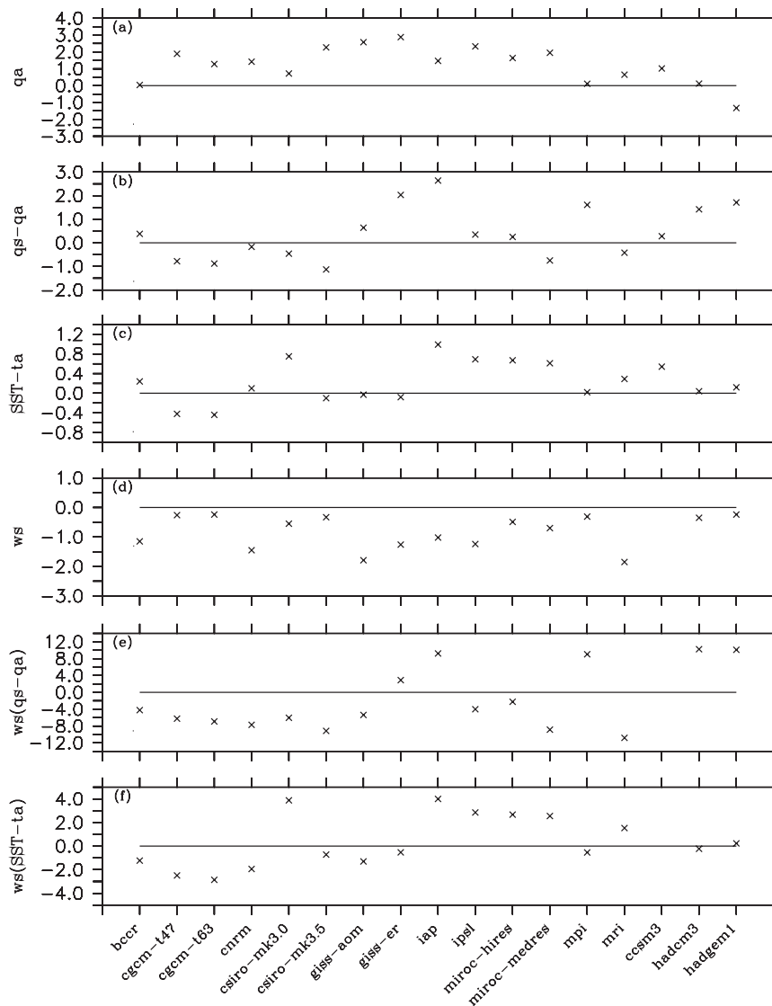
FIG. 5. Biases of (a) surface air specific humidity at 2 m ( q_a , \text{g kg}^{-1} ), (b) difference between the saturation and air specific humidity ( q_s , \text{g kg}^{-1} ), (c) difference between SST and air temperature at 2 m ( \text{SST} - T_a , ^{\circ}\text{C} ), (d) wind speed ( w_s , \text{m s}^{-1} ) at 10 m, (e) w_s(q_s - q_a) ( \text{m s}^{-1} \text{g kg}^{-1} ), and (f) w_s(\text{SST} - T_a) ( \text{m s}^{-1} ^{\circ}\text{C} ) in 17 IPCC AR4 coupled GCMs area averaged in 20^{\circ} – 5^{\circ}\text{S} , 100^{\circ} – 70^{\circ}\text{W} . Biases are computed relative to atmospheric and oceanic variables from the OAF flux monthly estimates during July 1983–December 1999; horizontal lines denote zero biases.
