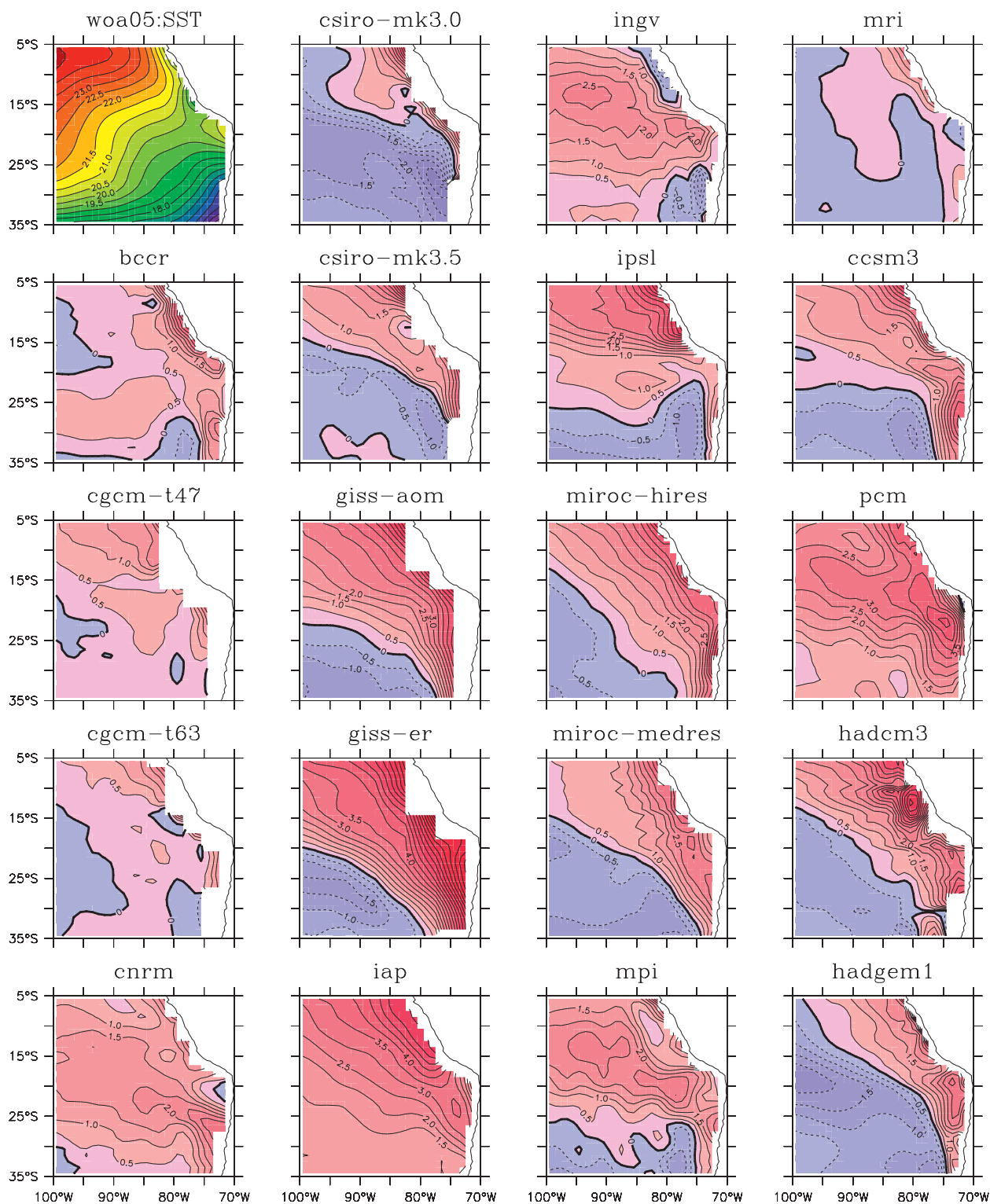
FIG. 1. Spatial distribution of the SST biases (shading contours; °C) relative to WOA05 from 19 IPCC AR4 coupled GCMs in the region (35°–5°S, 100°–70°W): (top left) SST from WOA05. Contour interval is 0.5°C.
