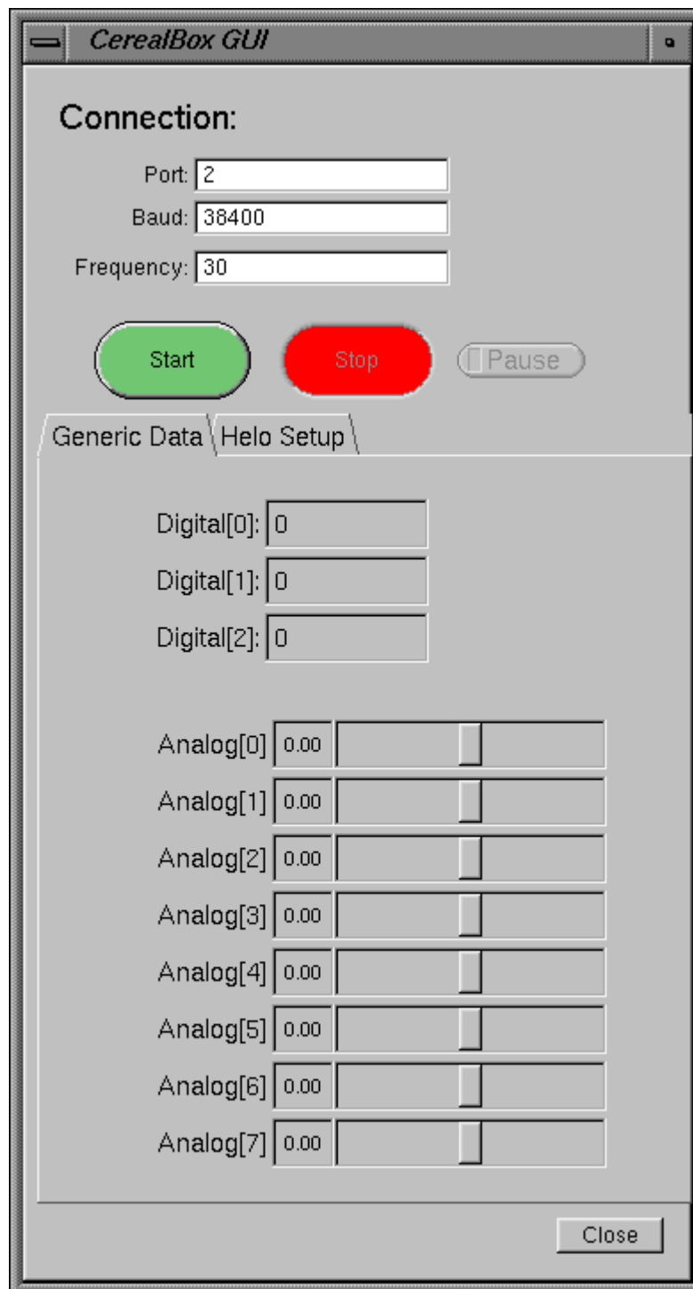
Figure 6 CerealBox Generic Data GUI Window
