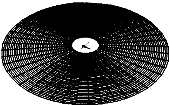
Figure 2: Far-field grid of observer points for the Kirchhoff acoustics simulation.
