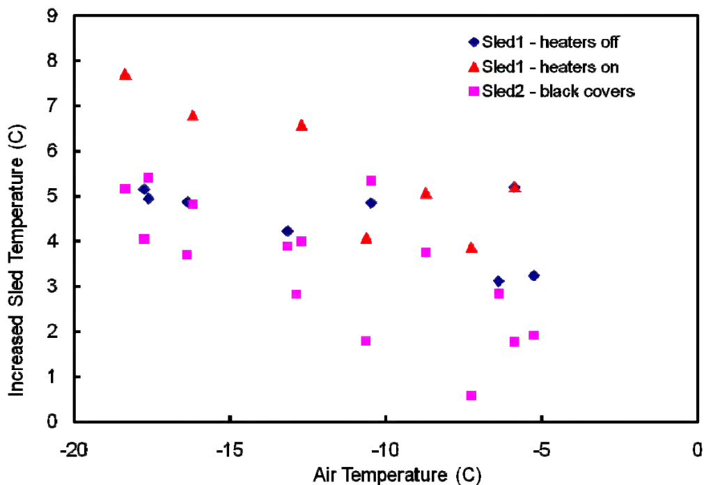
Figure 17. Increased steady state sled interface temperature versus air temperature for the three sled configurations tested. Heaters-on produced the largest warming benefit and black covers the least. The benefit for all configurations increased with colder air, a helpful effect probably related to frictional heating.
