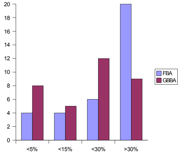
Figure 8: Histogram of L1 values for FBA and GBBA differences from the experimental data (smaller is better). For example, the 15-30% bin contains those scenes for which the predicted detection rate was off by between 15 and 30 percentage points.
