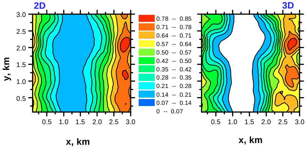
Fig. 2. Spatial distribution of the albedo field for the inhomogeneous cloud (right, 3D) and the vertically homogeneous cloud (left, 2D).
