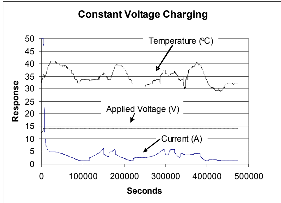
Figure 8. Charging profile of a 12V – 120Ah military grade VRLA battery.
