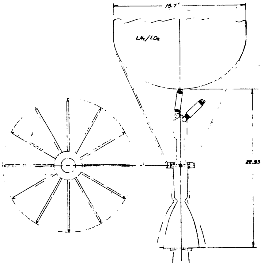
SINGLE-600K ENGINE GIMBALED ENGINE MT STRUCTURE - SKIRT, SKIN & STRINGERS
