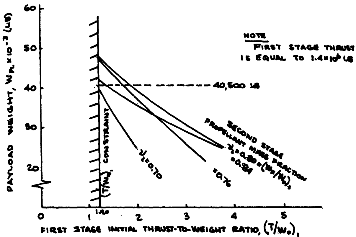
Figure 37. Payload Weight Versus First-Stage Initial Thrust-to-Weight Ratio for Solid/0.3 W'H
