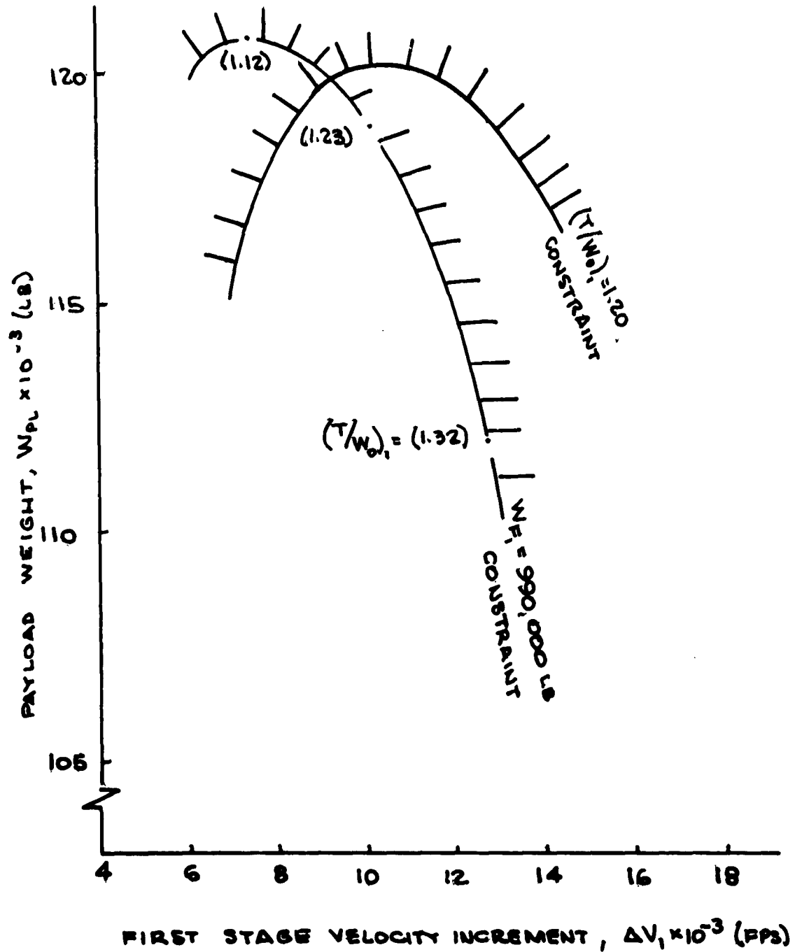
Figure 30. Payload Weight Versus First-Stage Velocity Increment for 3[2(0.3)WH]/2(0.3)W'H Module (Optimized Second Stage)
