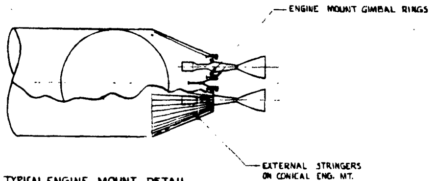
TYPICAL ENGINE MOUNT DETAIL FOR 2 P.W. ENGINES THRUST 300,000 LBS. EA.
