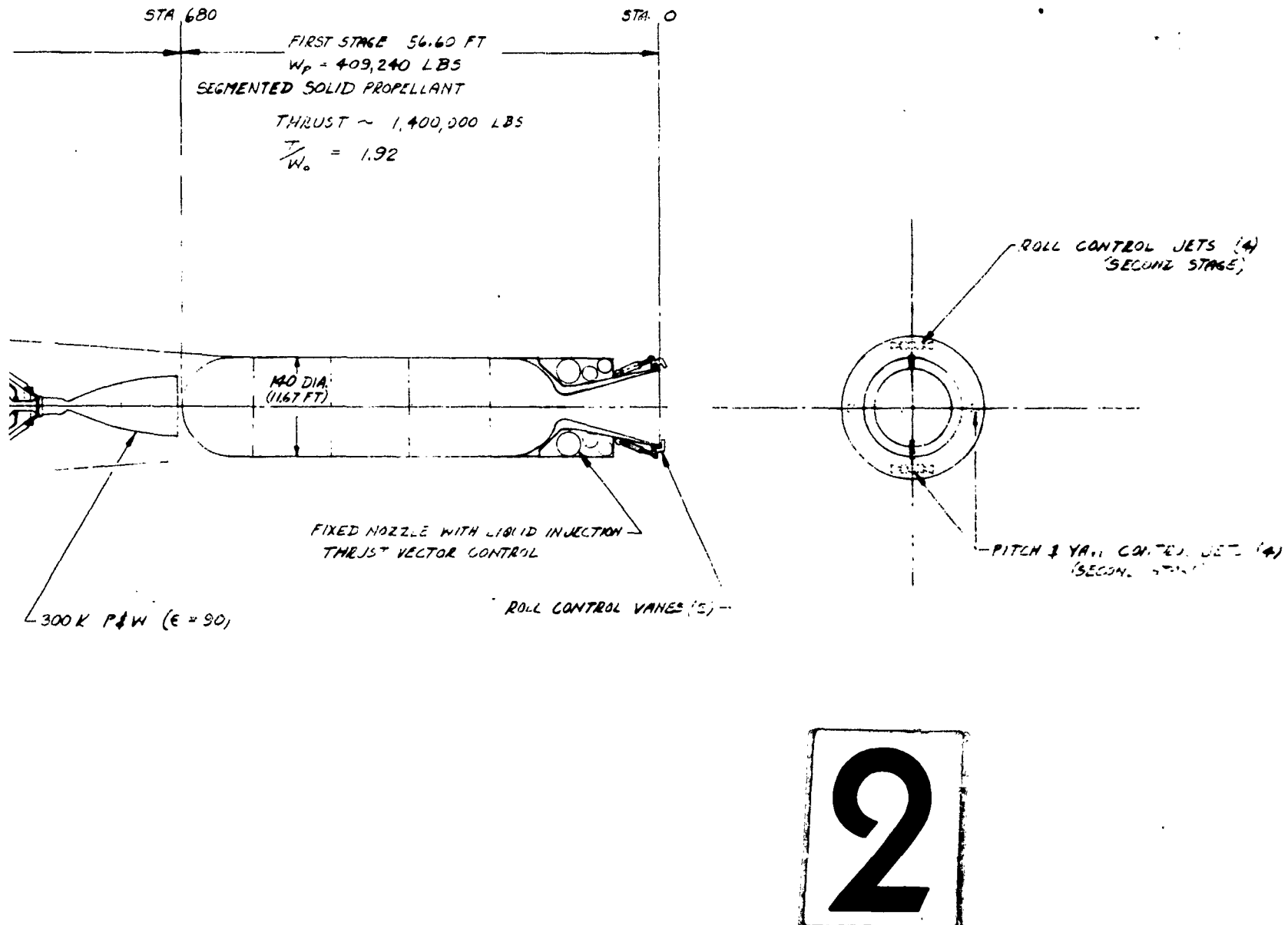
Figure A-9. 1.4M Solid First Stage - Pratt & Whitney 300K Liquid Oxygen Liquid Hydrogen Second Stage
