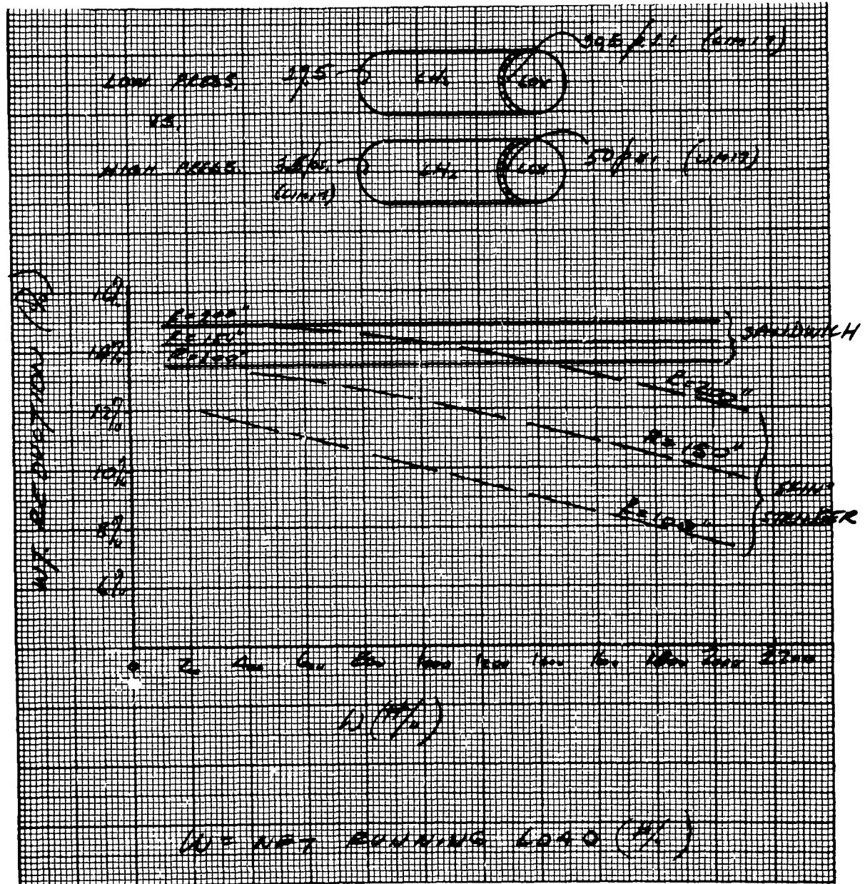
Figure 54. Liquid Hydrogen Liquid Oxygen Tankage Construction Comparison
