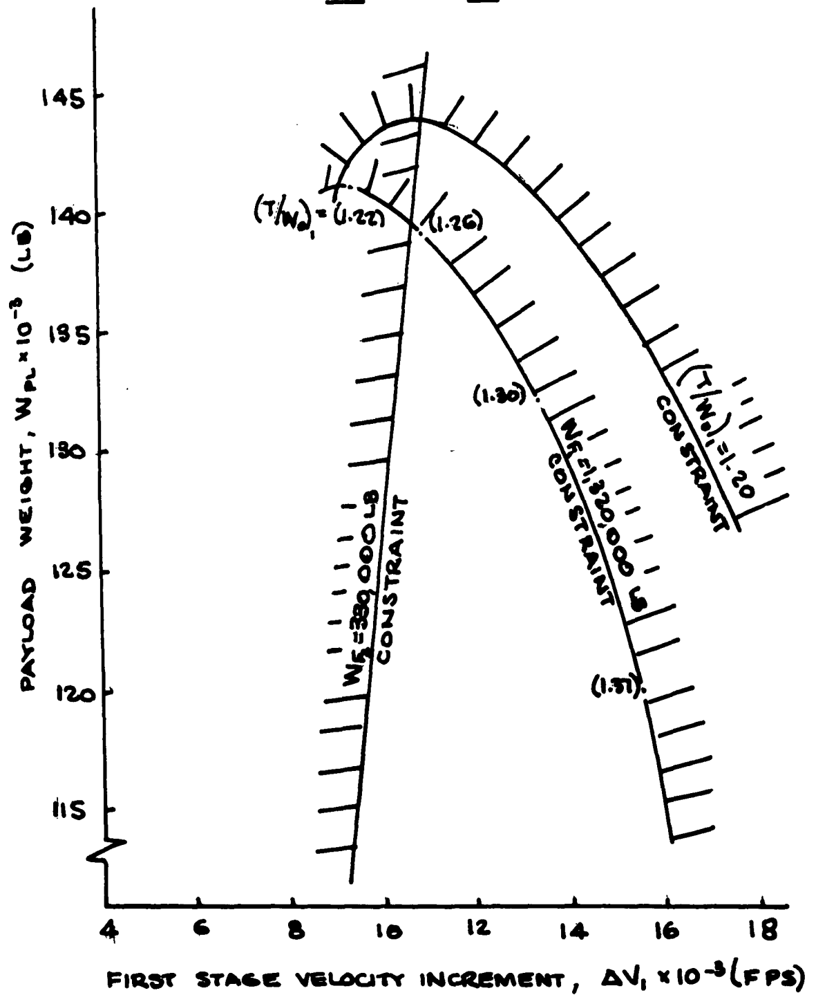
Figure 26. Payload Weight Versus First-Stage Velocity Increment for 4 [3(0.2WH)] / 3(0.2)WH Common Module
