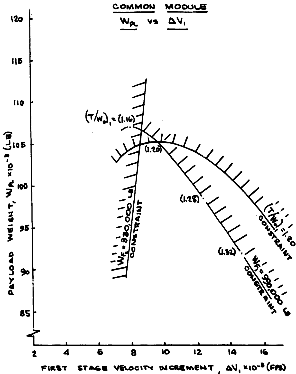
Figure 25. Payload Weight Versus First-Stage Velocity Increment for 3 [2(0.3)WH] / 2(0.3)WH Common Module
