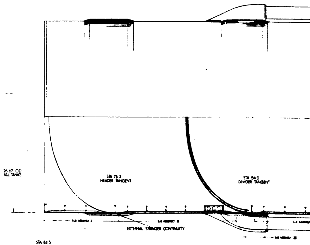
C-3 MODULAR ELEMENT (FROM BATTLE OMITTED)
