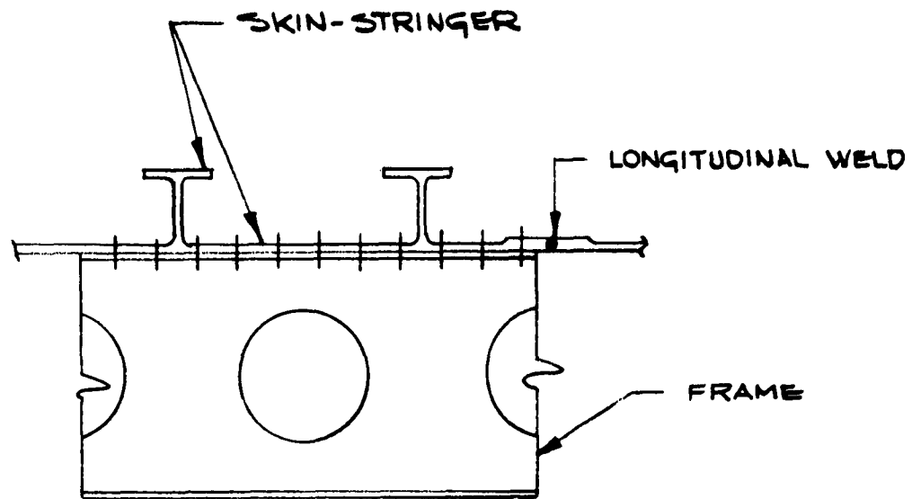
Figure 60. Typical Skin-Stringer Construction
