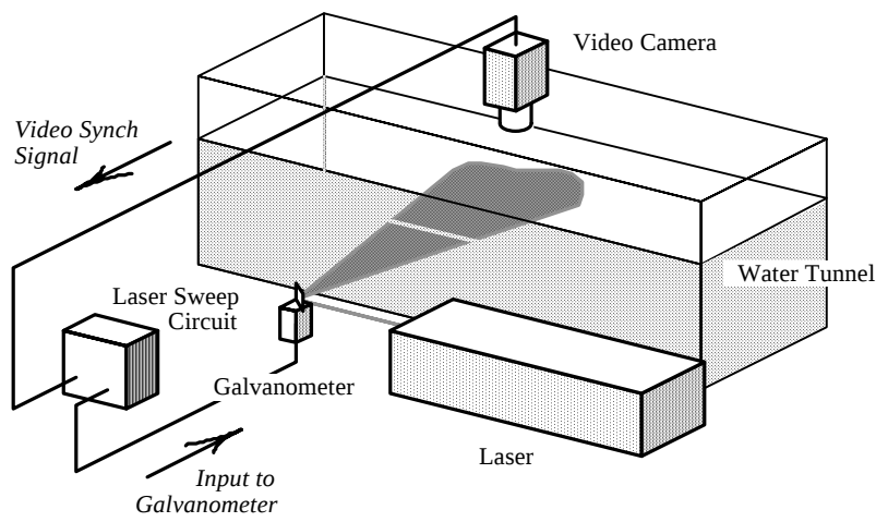
Figure 2. Oblique view drawing of the experimental the setup including optics, electronics, and water tunnel test section.
