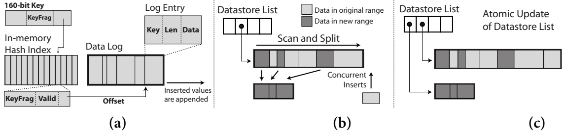
Figure 4.3: (a) FAWN-DS appends writes to the end of the Data Log. (b) Split requires a sequential scan of the data region, transferring out-of-range entries to the new store. (c) After scan is complete, the datastore list is atomically updated to add the new store. Compaction of the original store will clean up out-of-range entries.
