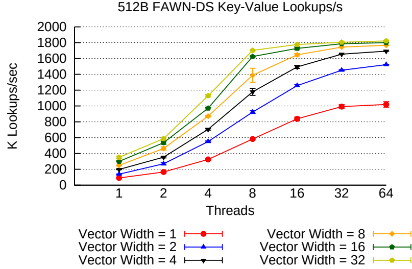
Figure 7.6: 512B synchronous read throughput through FAWN-DS using synchronous I/O interface. Multi-I/O allows applications using synchronous I/O to maintain a high queue depth at the device without requiring hundreds of threads.
