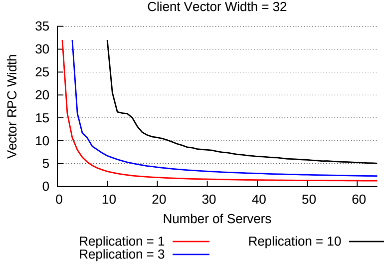
Figure 7.14: Simulation results showing the expected vector width of multiget RPCs, with the client making requests for 32 random keys, as a function of cluster size and replication factor. Data is assumed to be distributed evenly across all nodes, and replica nodes are chosen randomly (without replacement).
