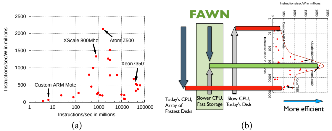
Figure 2.4: (a) Processor efficiency when adding fixed 0.1W system overhead. (b) A FAWN system chooses the point in the curve where each individual node is balanced and efficient.
