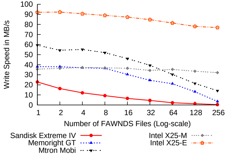
Figure 4.4: Sequentially writing to multiple FAWN-DS files results in semi-random writes.
