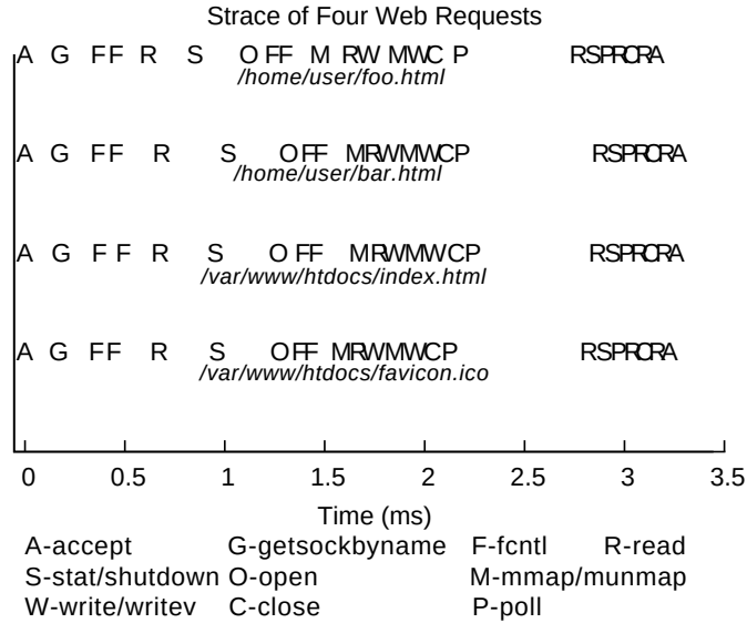
Figure 8.2: Trace of four different web requests serving static files shows the same system calls are always executed, and their execution paths in time are similar.
