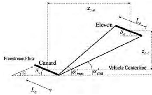
Fig. 12 Canard-elevon interactions.
