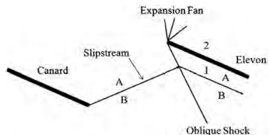
Fig. 13 Slipstream incident on elevon.
