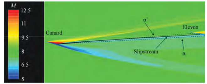
Fig. 22 Mach contours for canard-elevon horizontal distance 12c.
