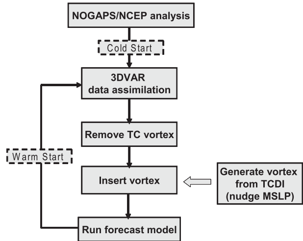
FIG. 2. Schematic of the TCDI system flow. Vortices are dynamically initialized to the minimum sea level pressure (MSLP) using the idealized model.
