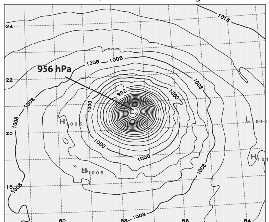
FIG. 4. Sea level pressure evolution (hPa) for the 0000 UTC 19 Aug warm start of Bill for the (a) control and (b) TCDI experiments on the 5-km COAMPS-TC domain with a horizontal scale of approximately 905 km.
