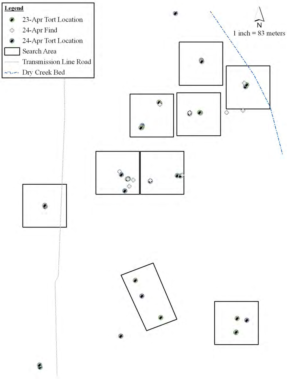
Figure B- 1. Tortoise location data for 23-24 April 2008 and search area delineation for 24 April 2008.
