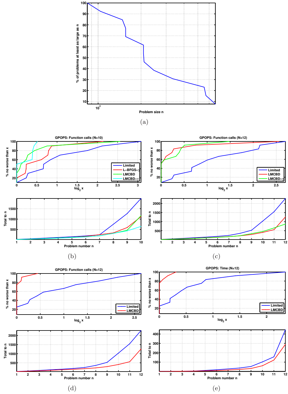
Figure 3.5: Results for SNOPT on the GPOPS example problems.
