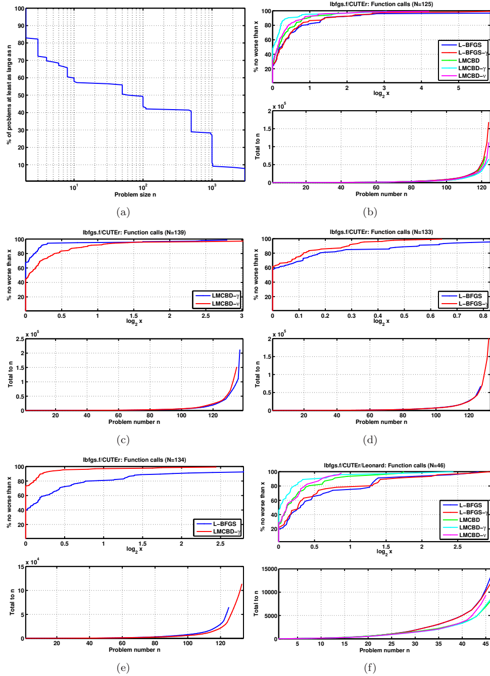
Figure 3.3: Results for the original and modified versions of lbfgs.f .
