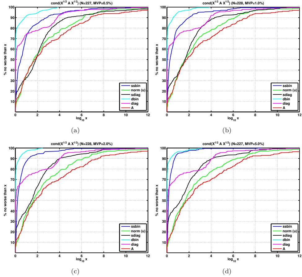
Figure 2.4: The performance of all methods for symmetric matrices. The title of each figure indicates the number of matrix-vector products and the performance metric. MVP = p\% means that \lfloor \frac{pn}{100} \rfloor matrix-vector products are used for a matrix of size n . In these plots, the performance metric is the condition number of the scaled matrix.
