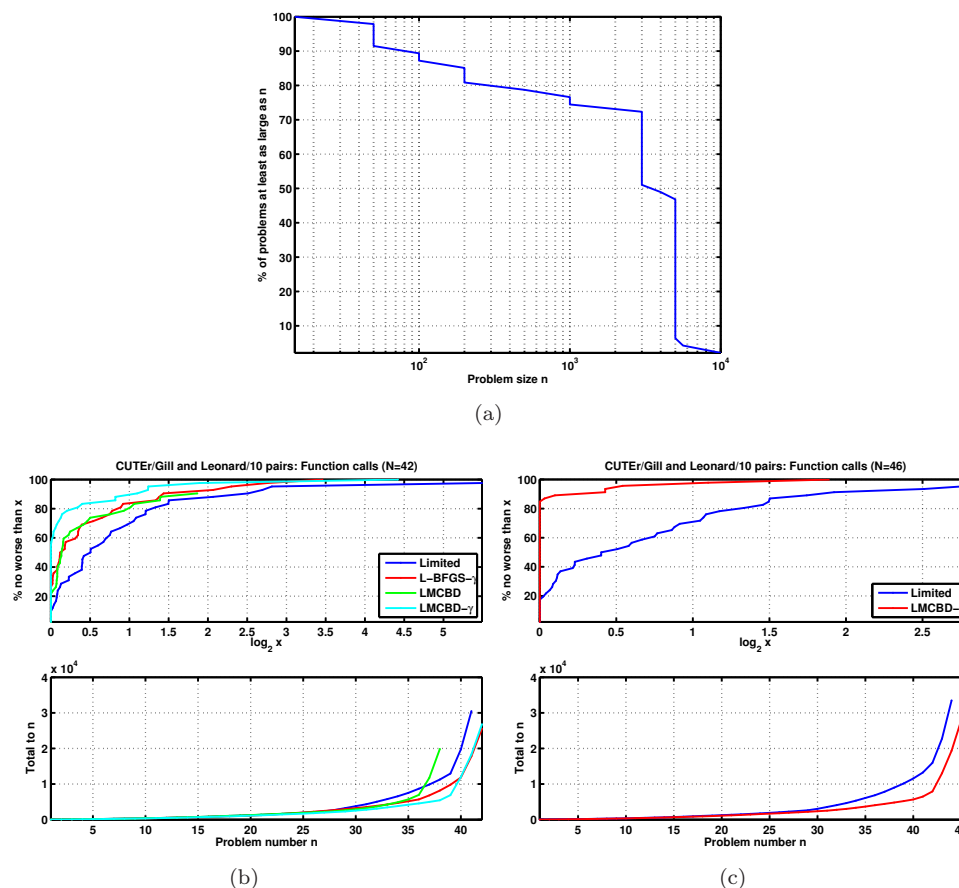
Figure 3.7: Results for SNOPT on the CUTer/Gill and Leonard test set.
