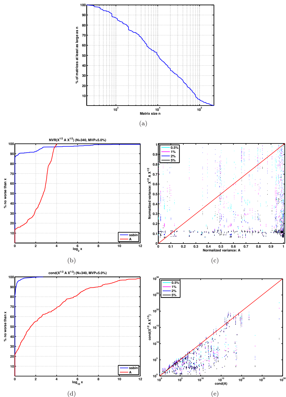
Figure 2.7: The performance of SBIN on symmetric matrices. (a) Matrix sizes. (b, c) The performance metric is the normalized variance of the row 2-norms (NVR). (d, e) The performance metric is the condition number.
