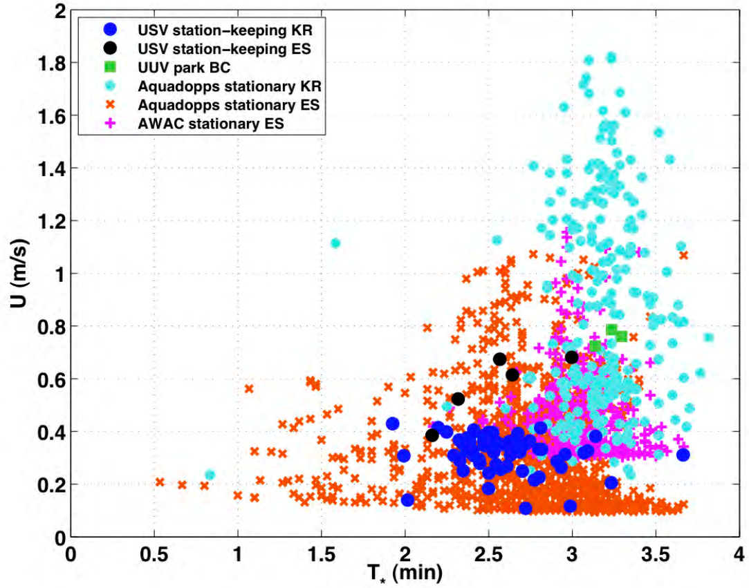
Figure 12. Depth-averaged flow velocity magnitude versus depth-averaged averaging window, T_* , measured by ADCPs mounted on various stationary platforms in differing environments.
