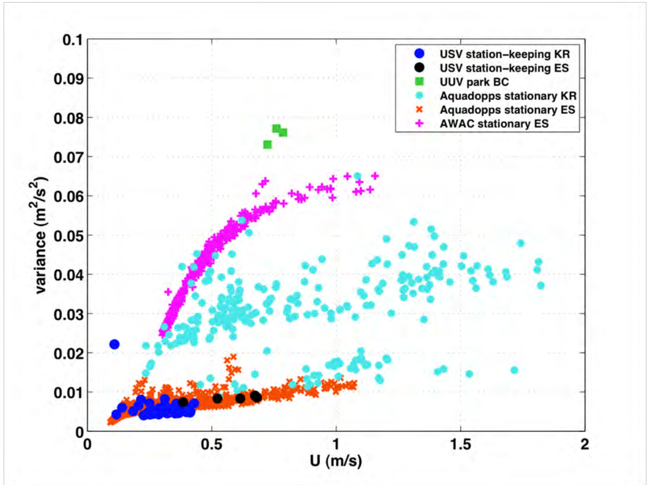
Figure 8. Depth-averaged flow velocity magnitude variance versus depth-averaged mean flow velocity magnitude measured by ADCPs mounted on various stationary platforms in differing environments.
