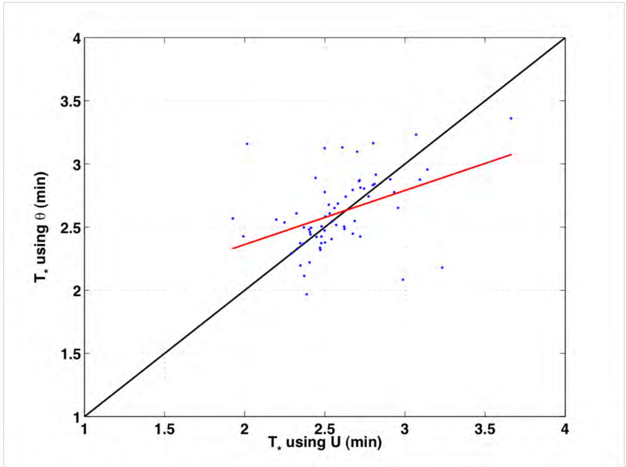
Figure 10. Correlation between T^* calculated using flow velocity magnitude ( U ) and T^* calculated using flow direction ( \theta ). The black solid line represents an idealized linear regression line and the red solid line represents the actual linear regression line for the comparison ( R^2=0.18 , m=0.43 ).
