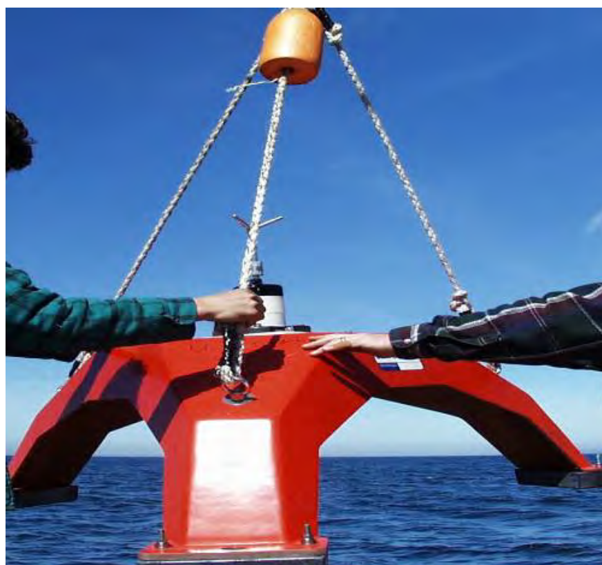
Figure 5. Tri-pod used for bottom-mounted upward-looking ADCPs
