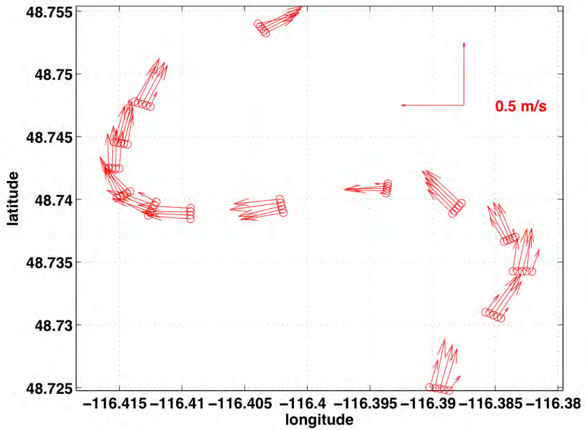
Figure 13. Spatial map of the velocity field in the meandering reach of the KR measured by the station-keeping USV.
