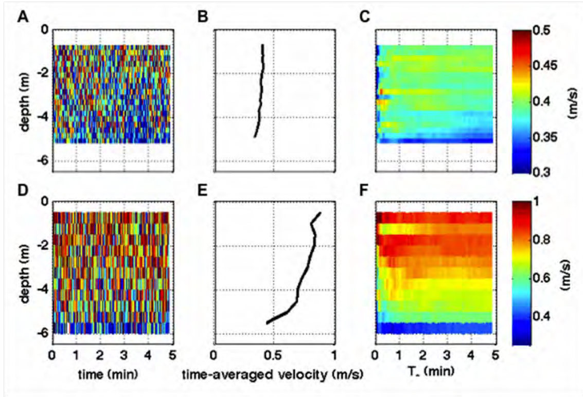
Figure 6. ADCP data collected by the station-keeping USV in KR (top row) and the UUV in "park" mode at BC (bottom row): (A,D) raw flow magnitude as a function of time and depth, (B,E) time-averaged vertical flow magnitude profiles, and (C,F) window-varying time averaged flow magnitude as a function of averaging window and depth. Colorbars represent flow velocity magnitude.
