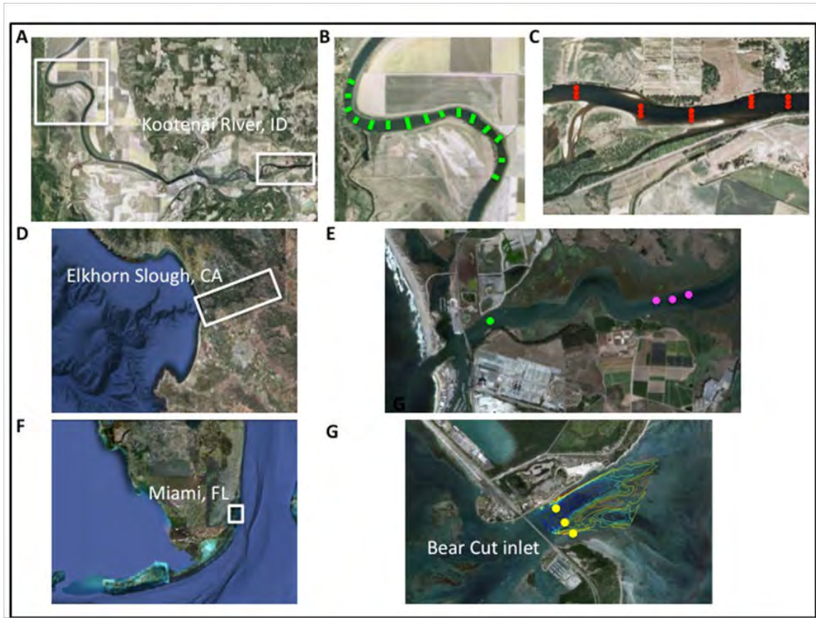
Figure 3. Experiment locations: (A) Kootenai River, ID, and view of (B) the meandering reach and associated USV transects, and (C) the braided reach and mini-catamaran locations; (D) Monterey Bay, CA, and view of (E) Elkhorn Slough including the USV stationary point (green dot) and the stationary ADCP locations (magenta dots); (F) Miami, FL, and view of (G) Bear Cut inlet and bathymetry obtained with the UUV and the UUV park locations
