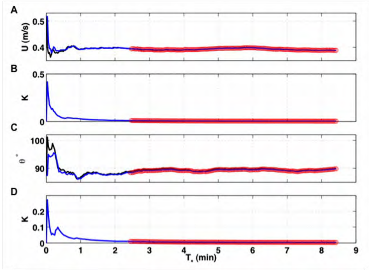
Figure 7. Values of (A) flow velocity magnitude estimated by the window-varying time average method (black) and by KA (blue), (B) velocity magnitude Kalman gain, K , (C) flow direction estimated by the window-varying time average method (black) and by KA (blue), and (D) direction Kalman gain, K , as a function of averaging window, T_* , for one ADCP bin from the station-keeping USV in KR. The red circles indicate when K < 0.01 and the estimate of the mean is considered stable.
