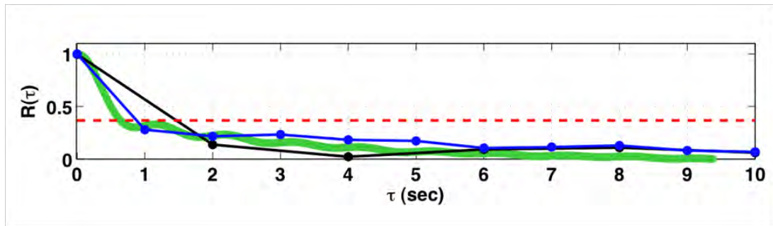
Figure 9. Autocorrelation functions as a function of time lag, \tau , for U measured by: the station-keeping USV in KR with dt=2 s (black), an Aquadopp in KR with dt=1 s (blue), and the ADV in KR with dt=1/32 s (green), where the red dashed line represents the decorrelation criteria ( 1/e ).
