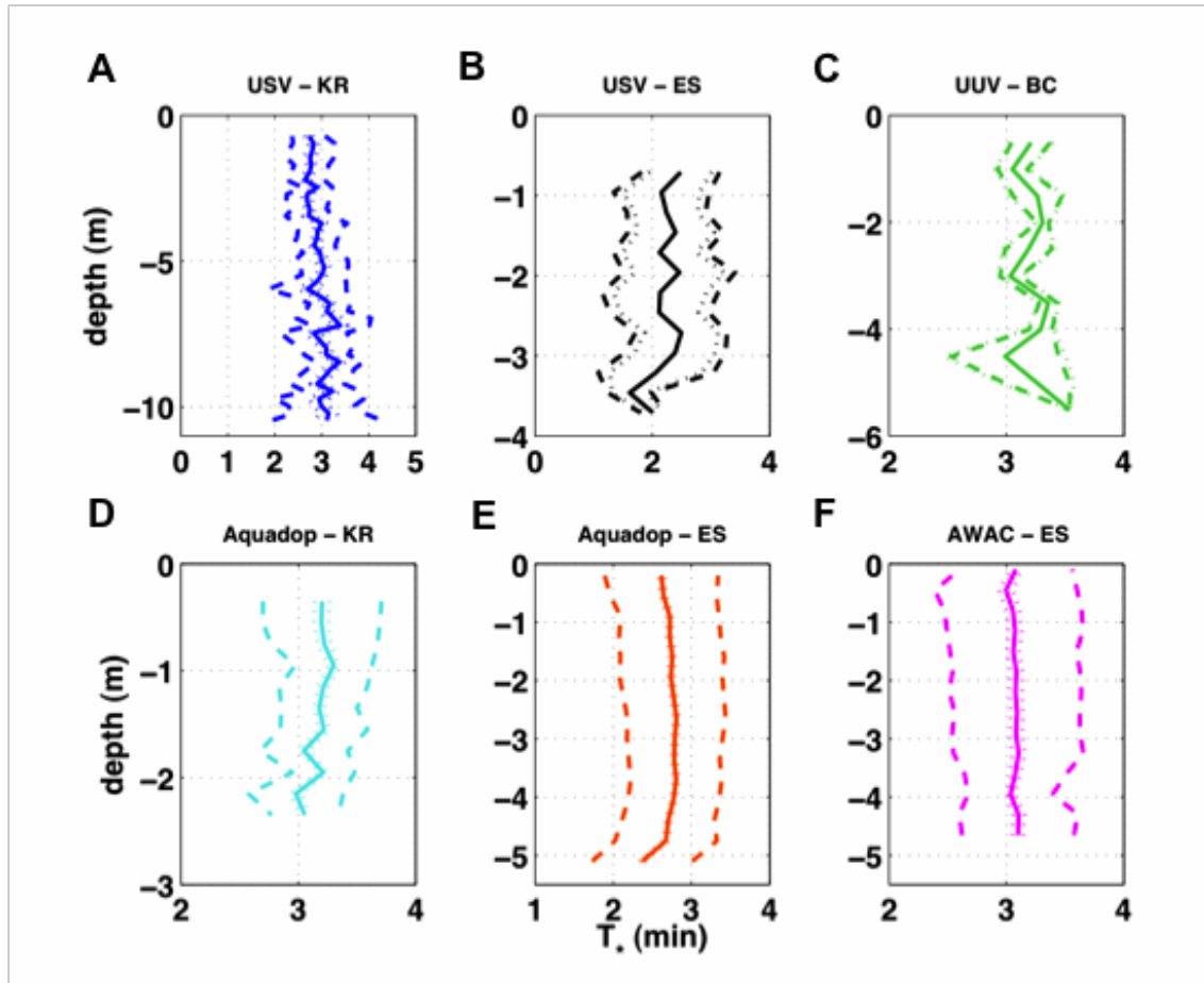
Figure 11. Averaging window, T^* , as a function of depth, determined for (A) the station-keeping USV at KR, (B) the station-keeping USV at ES, (C) the UUV in “park” mode at BC, (D) stationary downward-looking Aquadopps at KR, and for the fixed bottom-mounted (E) Aquadopps and (F) AWAC in ES. Note that all ADCPs were stationary. Solid lines depict the mean averaging window, dashed lines depict one standard deviation, and dotted lines depict the 95% confidence level.
