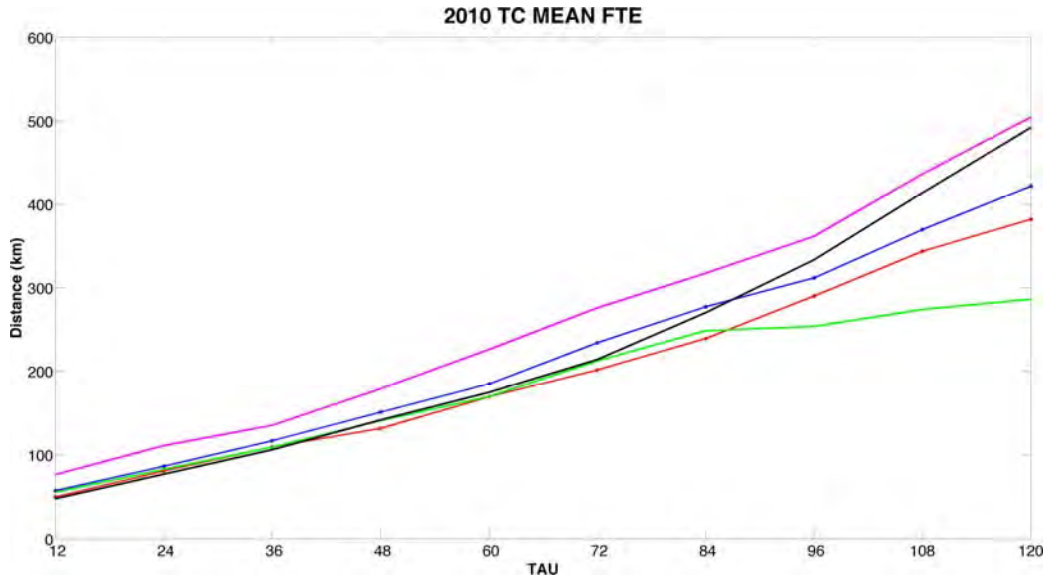
Figure 11. The EPS mean FTE from 12 h to 120 h forecast intervals. The MORGREPS mean is in magenta. The GFS mean is in black. The ECMWF mean is in green. The GE mean is in blue. The consensus mean is in red.
