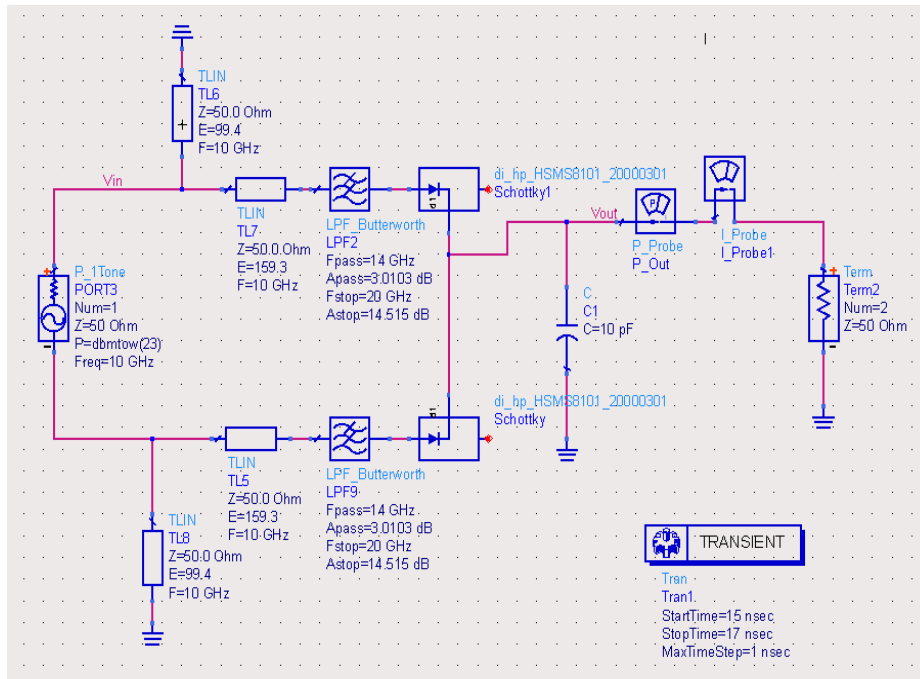
Figure 38. ADS model of a full-wave rectenna design with a pre-LPF.
