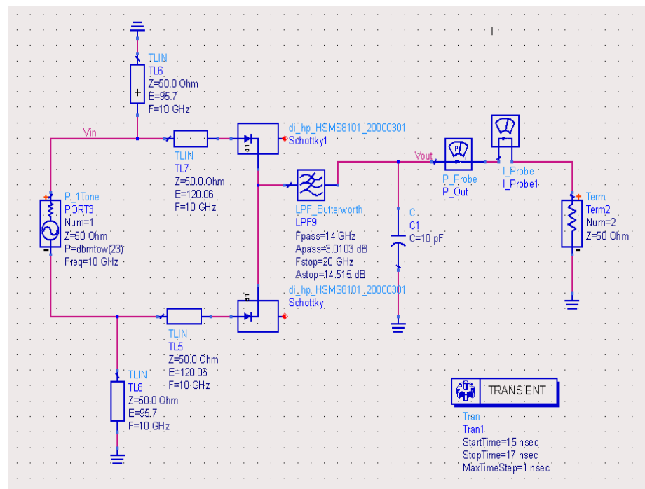
Figure 39. ADS model of a full-wave rectenna design with a post-LPF.
