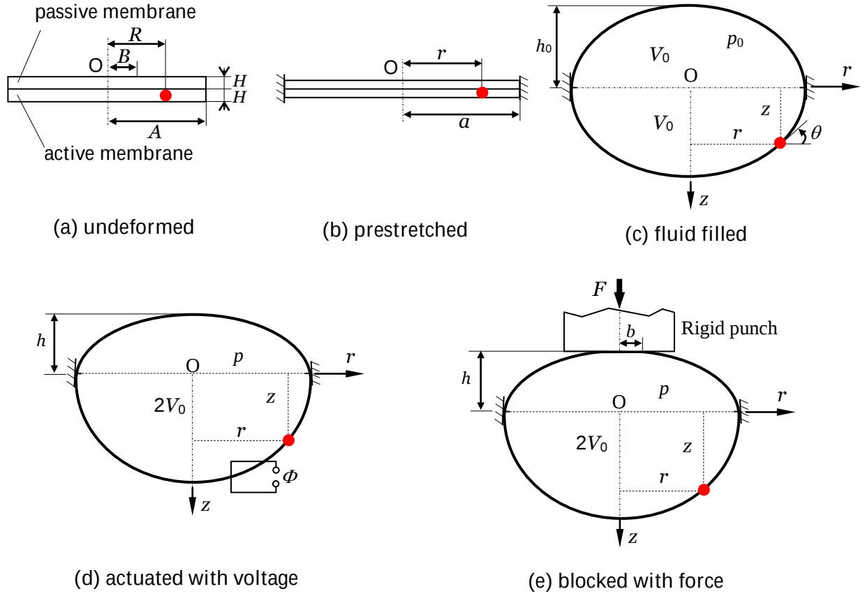
FIG. 3. Schematics of states used to describe the computational model. In each state, the position of a particular material particle has been identified by a red dot.
