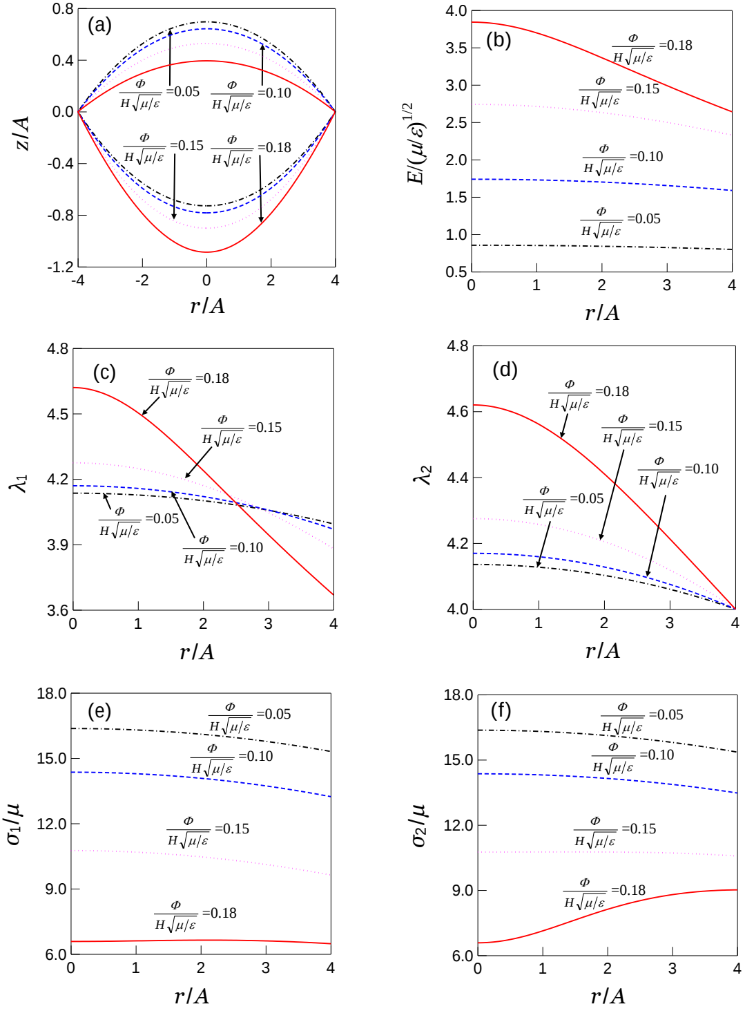
FIG. 6. Distribution of various fields in the active membrane at several values of the voltage. (a) Deformed shapes of the actuator. (b) True electric field. (c) Longitudinal stretch. (d) Latitudinal stretch. (e) Longitudinal true stress. (f) Latitudinal true stress.
