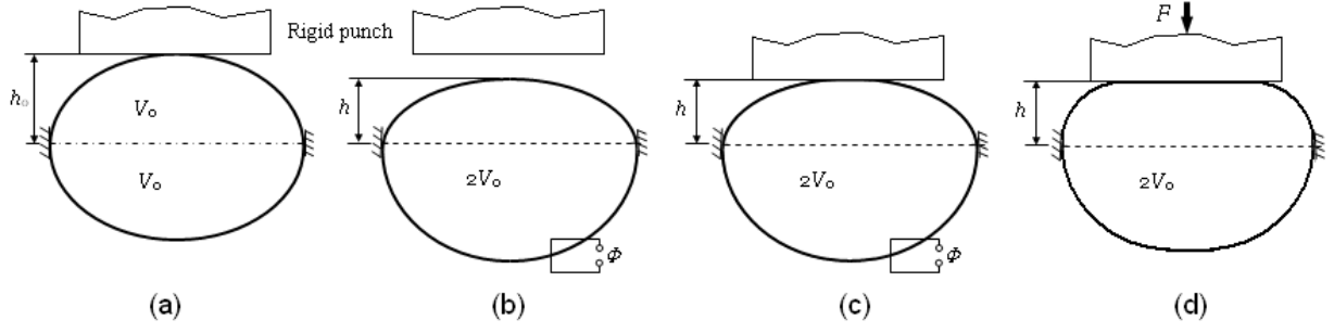
FIG. 2. Experiment to characterize the HCDE actuator. (a) While the actuator is in the rest state, a rigid flat punch is brought to touch the top membrane with negligible force. (b) When the bottom membrane is subject to voltage, both membranes move downward. (c) While the voltage is on, the rigid punch is brought to touch the top membrane with negligible force, and the displacement of the punch defines the free stroke. (d) The voltage is turned off while the punch is fixed in position, the punch presses the top membrane over an area of contact at a certain blocking force.
