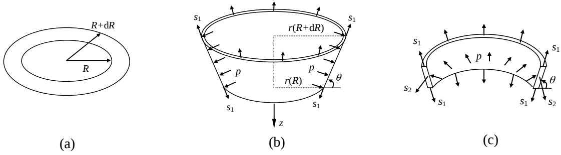
FIG. 4. Free-body diagrams to describe the mechanical equilibrium of a membrane. (a) In the undeformed state of the membrane, imagine an annulus, radii R and R+dR . (b) In a deformed state, the annulus becomes an axisymmetric band. The pressure on the face of the band is balanced by the longitudinal stress on the rims of the band. (c) Balance the pressure, the longitudinal stress, and the latitudinal stress in a half of the band.
