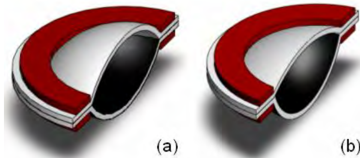
FIG. 1. Sectional views of a hydrostatically coupled dielectric elastomer (HCDE) actuator. Two membranes of a dielectric elastomer are clamped by rigid circular rings. The bottom membrane is sandwiched between soft electrodes, which are connected to a voltage source. Confined in between the membranes is a certain volume of a fluid. (a) When the voltage is off, the actuator is in the rest state. (b) When the voltage is on, the bottom membrane expands in area and moves downward, pulling the top membrane down through the coupling fluid.
