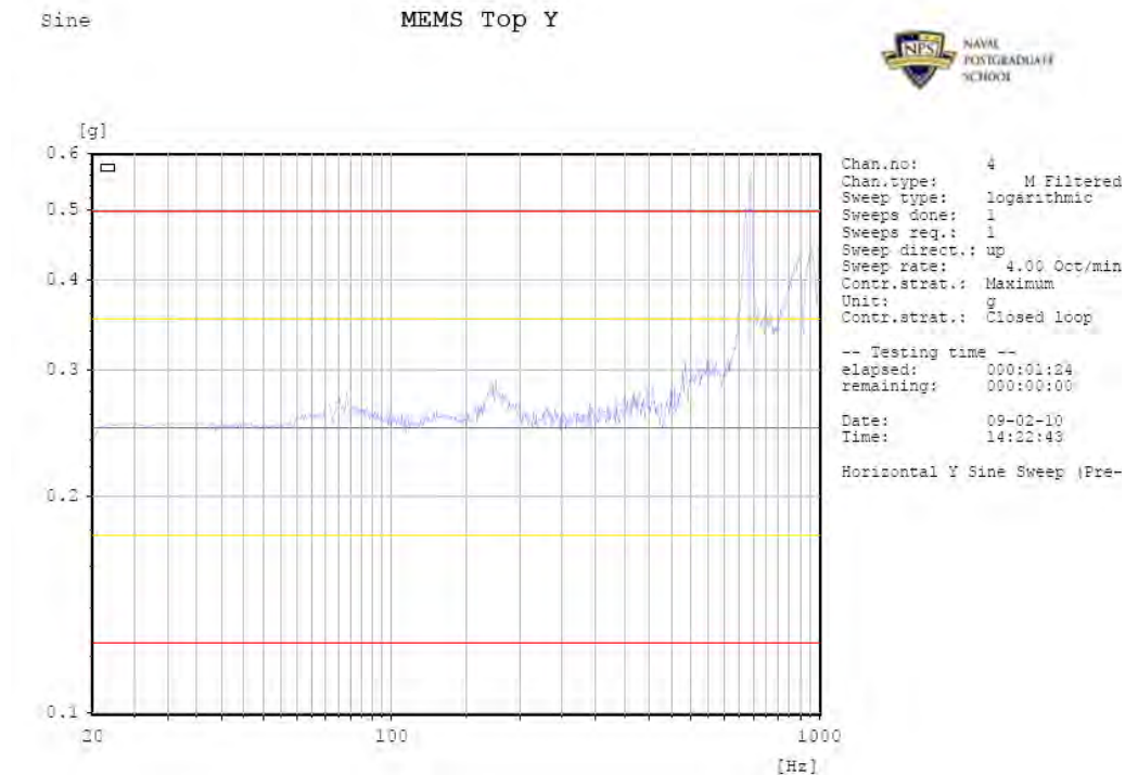
Figure 50. Low-level Sine Sweep (Pre-Random vbe) along the Y-Axis
