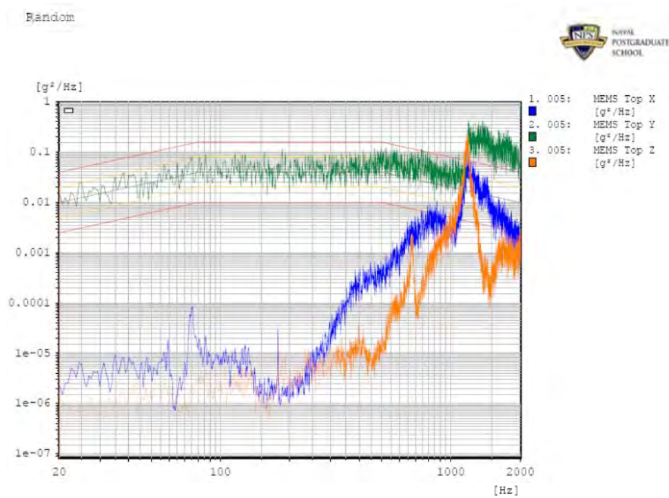
Figure 51. Random Vibration along the Y-Axis
