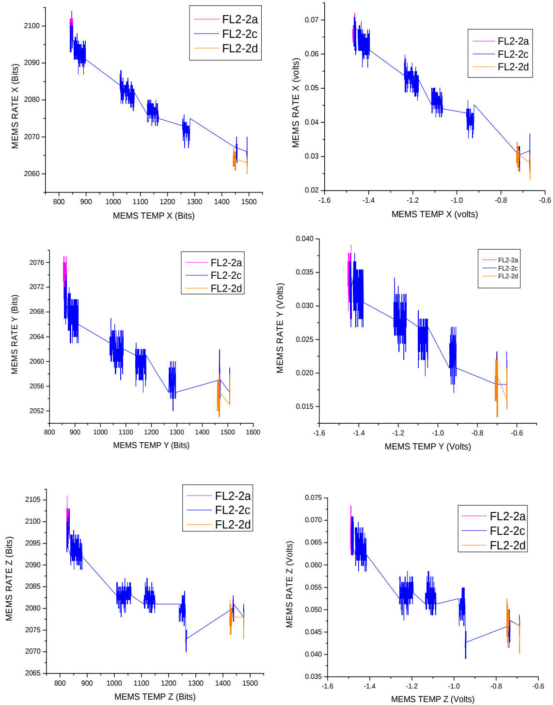
Appendix Figure 17. Hysteresis Test, FL2-1 (X,Y,Z)
