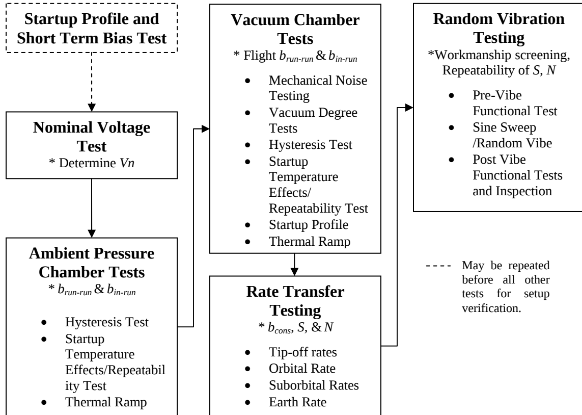
Figure 8. Test Flow
