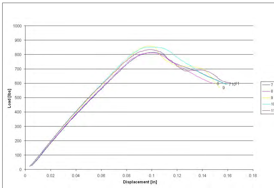
Figure 11: Sample Failure Plot of 8.41 Lb/Ft 3 , Half-Inch Thick Titanium Core Panel
