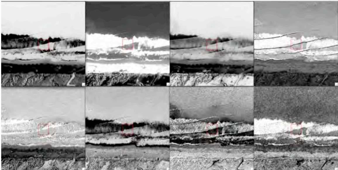
Figure 23. Eight Principal Component Bands for image P007
