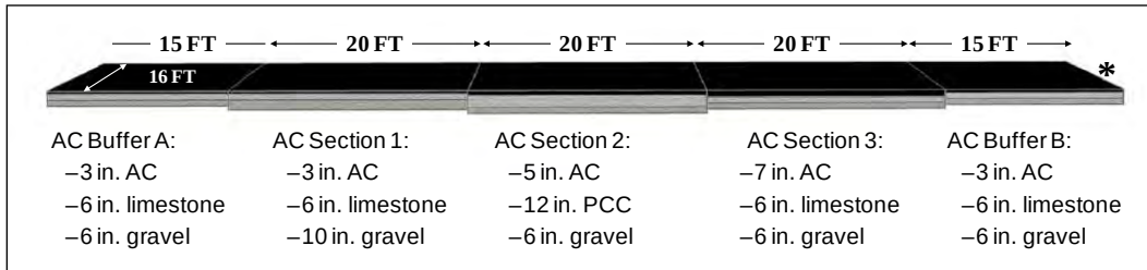
Figure 2. Layers of the AC portion of the custom test section. The * denotes where the AC and PCC sections connect.
