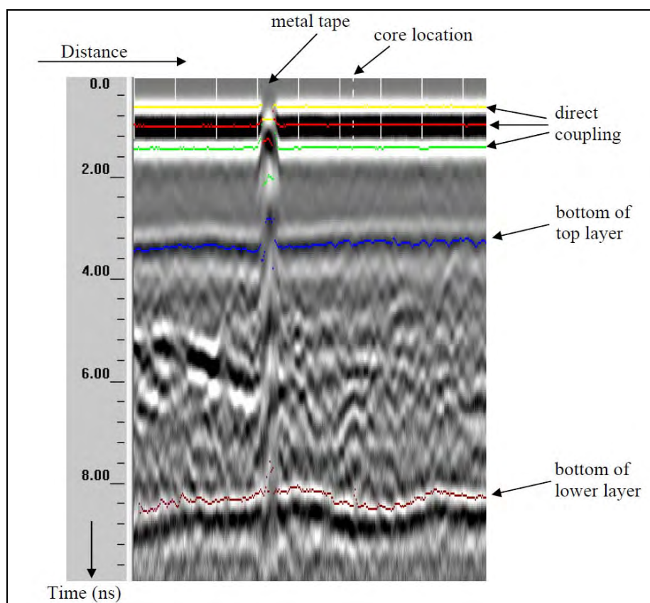
Figure 24. Example of the single ground-coupled GPR data from test location 8 (figure taken from Infrasense, Inc. 2010).
