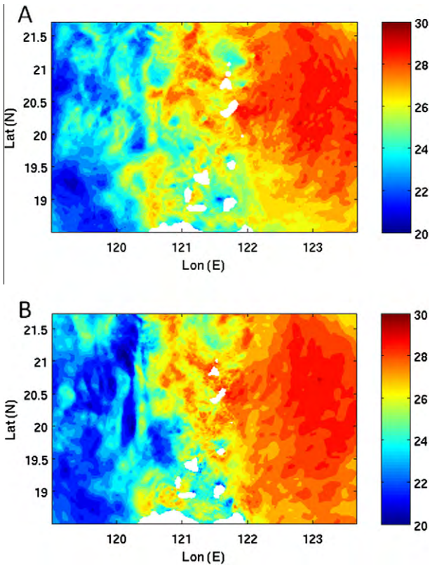
Fig. 6. (A) Temperature from inner domain solution and (B) outer domain solution cropped to inner domain area (bottom panel) at 95 m for hour 221.
