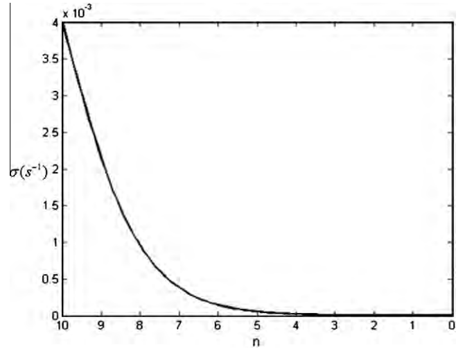
Fig. 1. Schematic of the relaxation zone at western boundary showing value of \sigma(n) where n is the coordinate normal to the boundary and width of relaxation zone ( \delta = N\Delta n , N = 10 ) gridpoints). Similar relaxation zones exist inside each of the four lateral boundaries between the inner domain and the outer domain.
