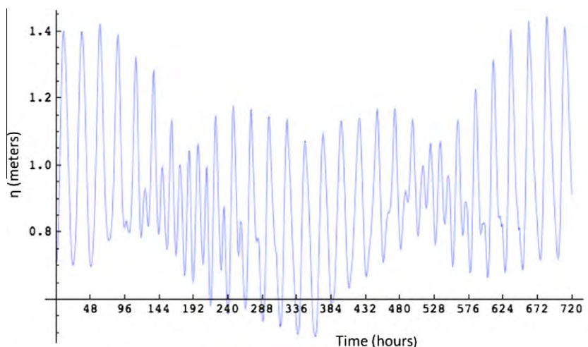
Fig. 3. Average sea surface height, \bar{\eta} , after application of the Transport Correction Scheme (TCS). The smaller range of \bar{\eta} indicates improved volume conservation. The tidal signal, which is a strong component of the forcing in this area, is now clearly visible.
