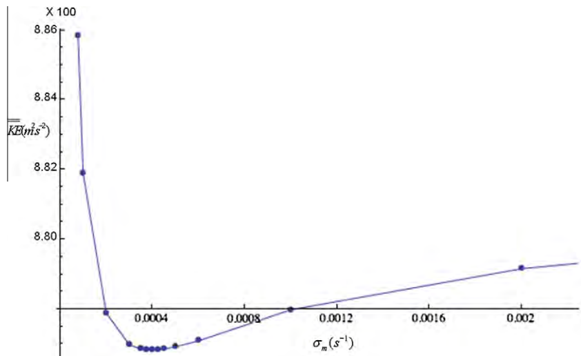
Fig. 5. Average horizontal kinetic energy ( \overline{KE} ) as a function of the maximum absorption parameter ( \sigma_m ).
