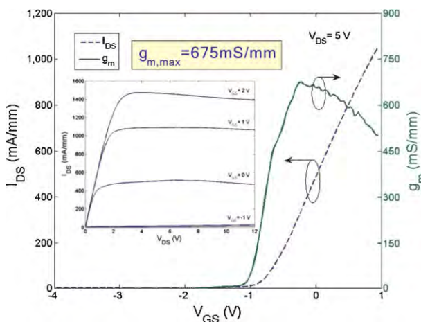
Figure 7 (online color at: www.pss-a.com ) Transconductance curve of a gate recessed AlInN/GaN HEMT ( L_G = 0.15 \mu\text{m} , 25 nm \text{Al}_2\text{O}_3 passivation) with a record peak extrinsic transconductance of 675 mS/mm. The insets show I_{DS,\text{max}} at different V_{GS} .
