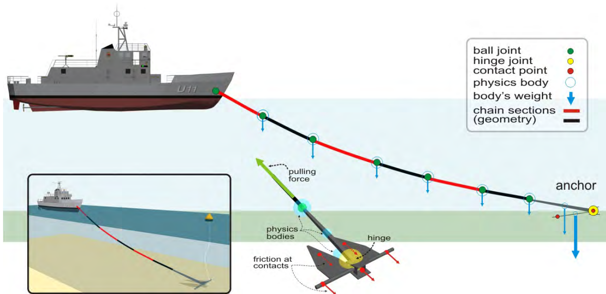
Figure 37. A graphical representation of the anchor and chain model
