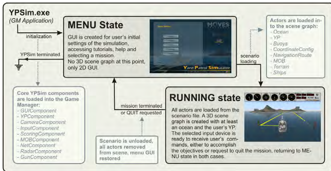
Figure 15. High-level view of YPSim's state cycle.
