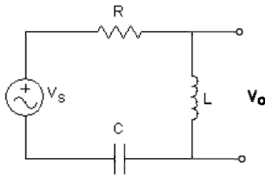
Figure 14: Circuit Model
