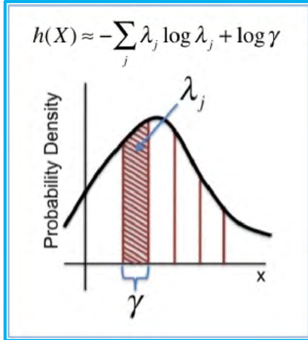
Figure 10: Entropy Estimation Method
