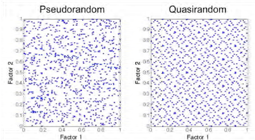
Figure 7: Comparison of Uniform Pseudorandom and Quasirandom Samples
