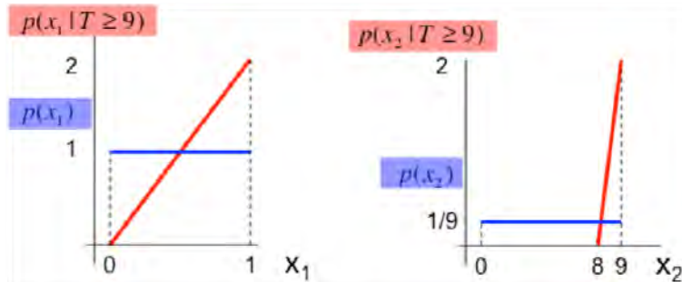
Figure 12: Unconditional and Conditional Distributions
