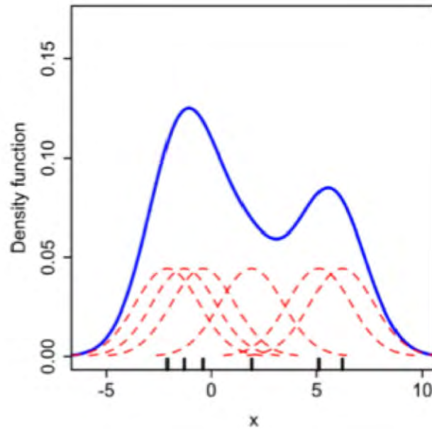
Figure 9: Notional Kernel Density Estimation of a Probability Density Function
