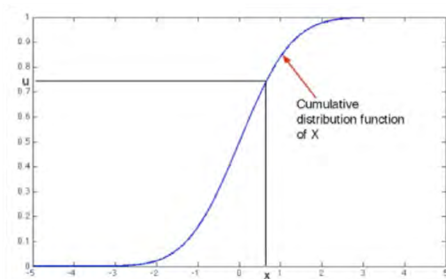
Figure 8: Cumulative Distribution Function Method for Sample Generation
