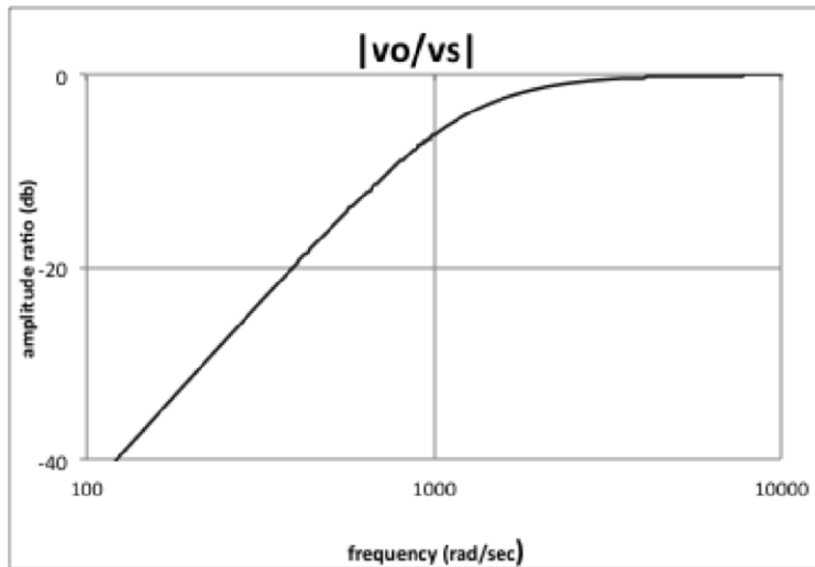
Figure 15: Frequency response
