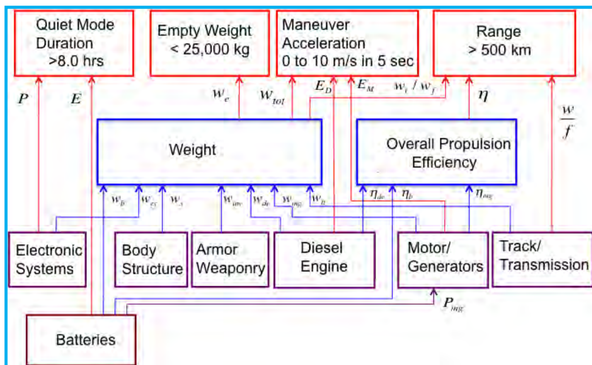
Figure 17: Simplified Work Break Down for an Infantry Fighting Vehicle
