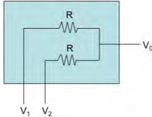
Figure 2: Adder Circuit
