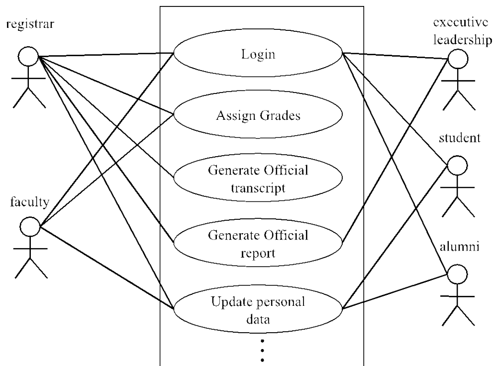
Figure 21. Refined Use Case Diagram
