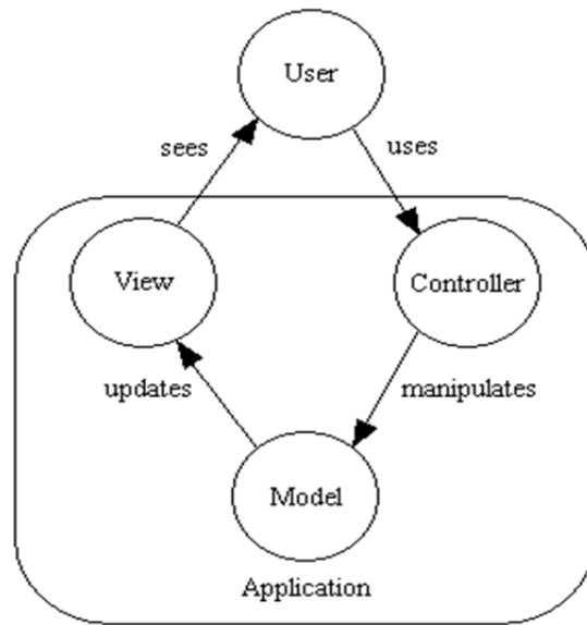
Figure 2. Traditional MVC Mapping. (From Joomla, 2010)
