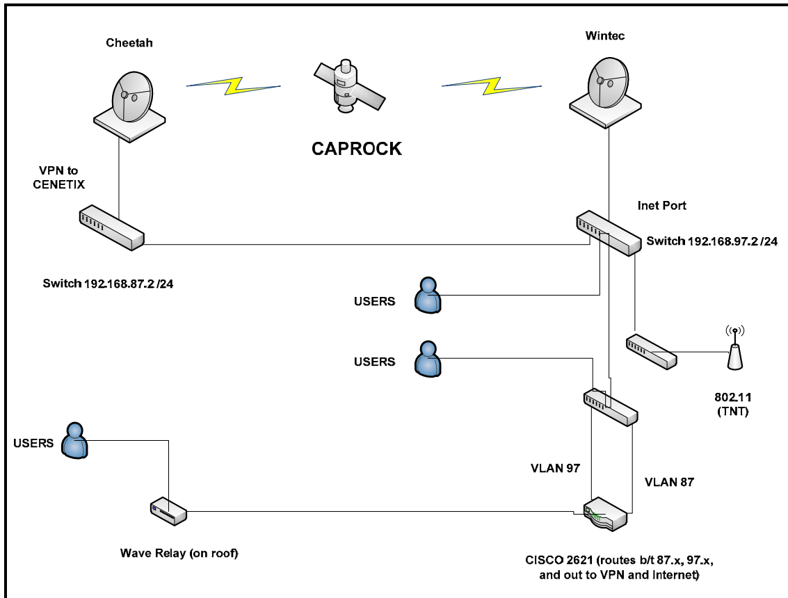
Figure 20. Detailed Diagram of Internal Network at Avon Park, FL
