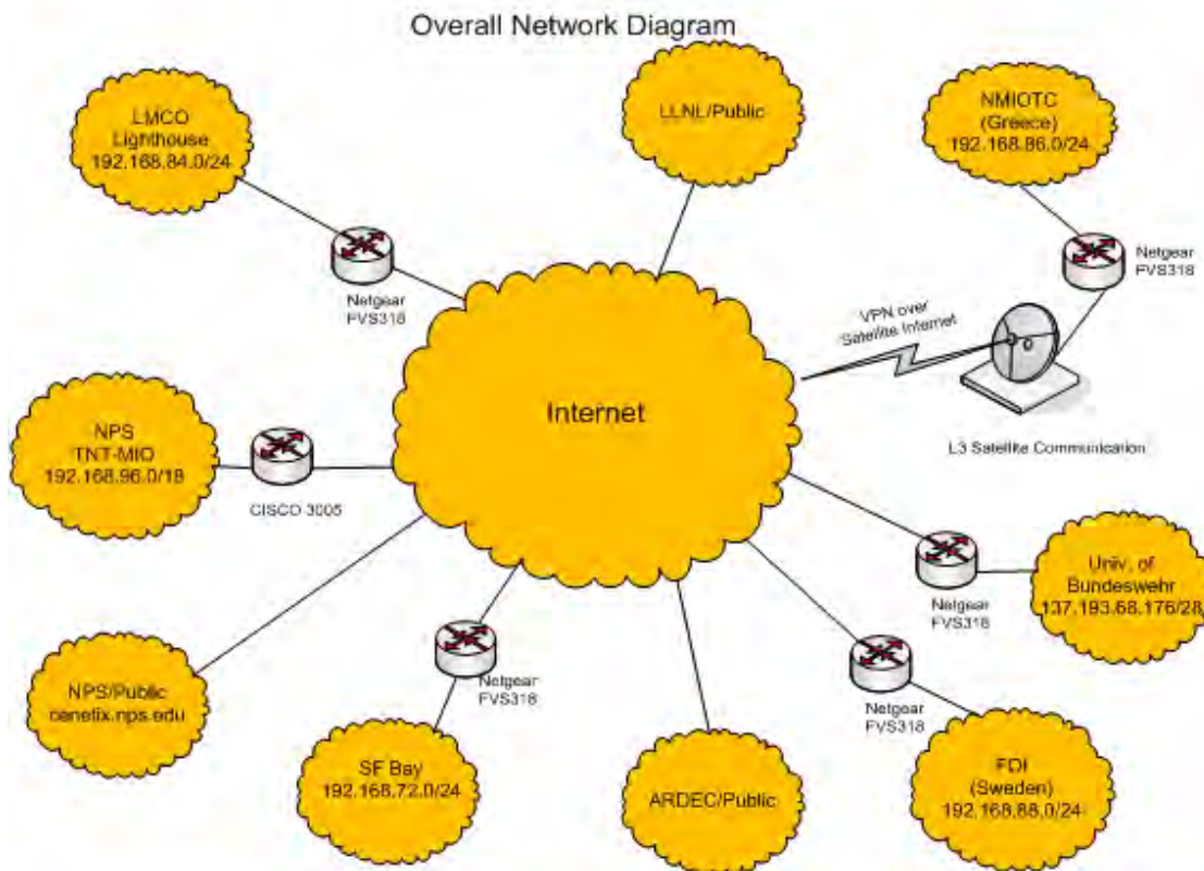
Figure 28. MIO Testbed Reachback and Detection Extended Network Basic Diagram (From TNT MIO, 2011, p. 50)
