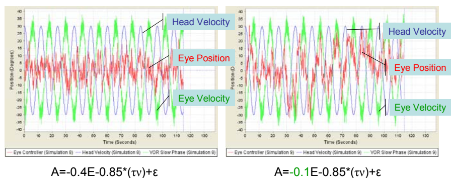
Figure 8: Long term effect of “fast phase” amplitude for cosine wave input
