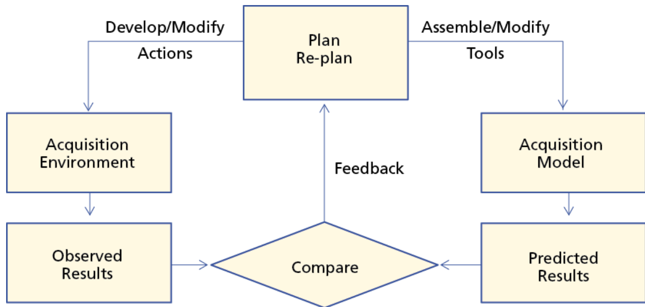
Figure 5-5. Plan to Re-plan Pattern
