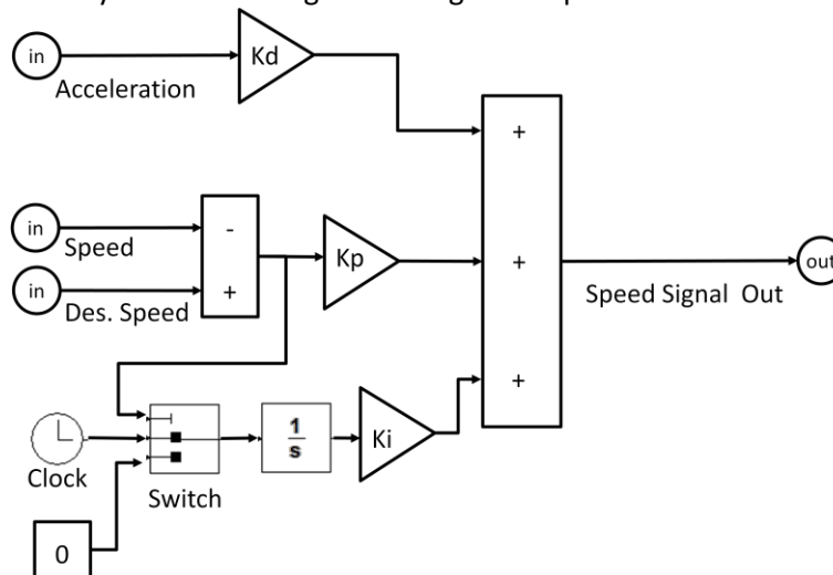
Figure ii - Speed Control
