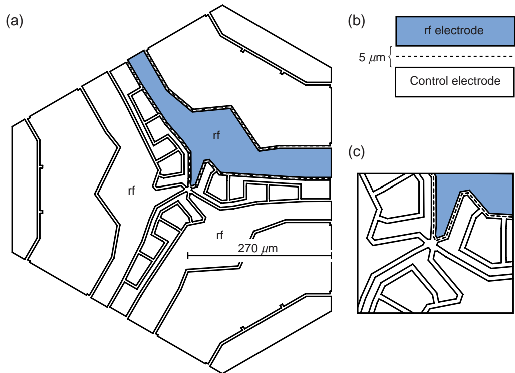
Figure 6. (a) The junction design used in the component library. The coordinates given in table 1 correspond to the dashed line around the shaded rf rail. (b) This perimeter is centered on the 5 \mu\text{m} gap between the rf rail and the control electrodes. (c) Detail of the center of the junction.
