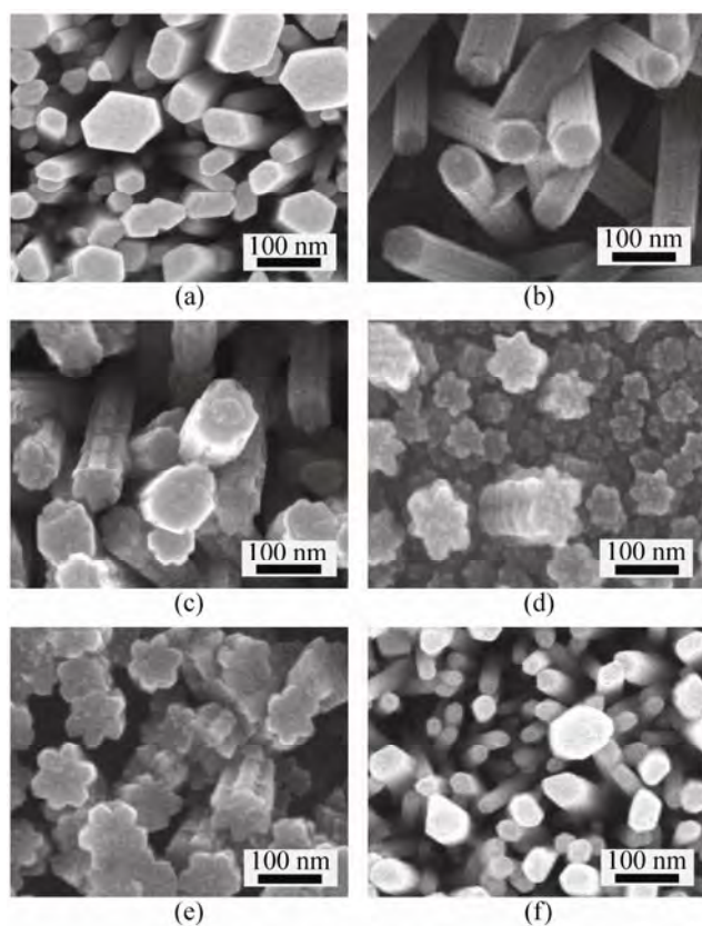
Figure 1 SEM images of ZnO nanostructures synthesized from the mixed aqueous solutions of 0.025 mol/L zinc nitrate and 0.025 mol/L hexamine with (a) no thiourea, (b) 0.025 mol/L thiourea, (c) 0.05 mol/L thiourea, (d) 0.1 mol/L thiourea, (e) 0.2 mol/L thiourea, and (f) 0.1 mol/L urea as a control sample
