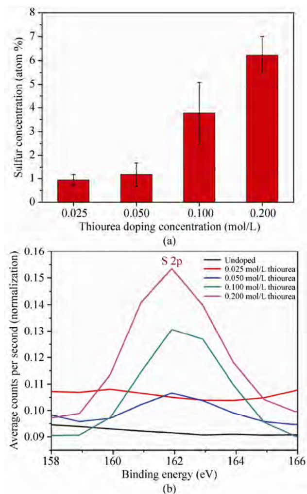
Figure 2 (a) Averaged sulfur concentrations obtained by XPS of various thiourea-doped ZnO nanostructures; (b) averaged core-level XPS corresponding to the sulfur 2p peak for ZnO nanostructures with various concentrations of thiourea. Black, red, blue, green, and pink lines indicate undoped, 0.025 mol/L, 0.050 mol/L, 0.1 mol/L, and 0.2 mol/L thiourea doped samples, respectively
